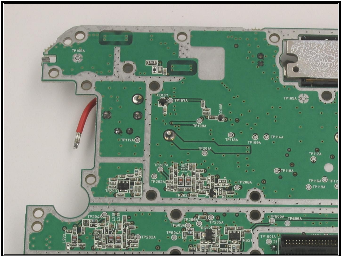
PHOTOGRAPH 26: TRX SYN BOARD SOLDER SIDE, UPPER LEFT
