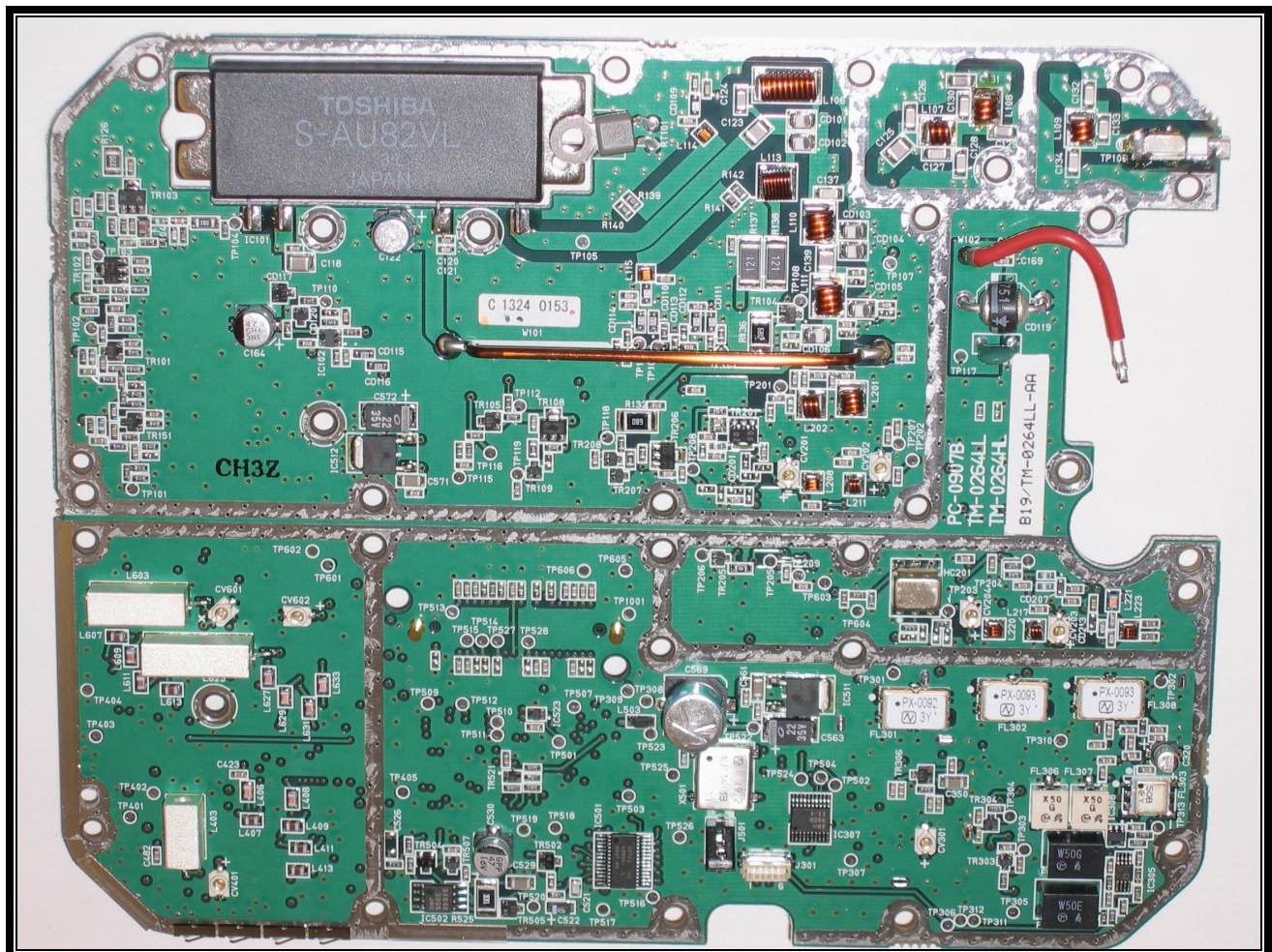
PHOTOGRAPH 18: TRX SYN BOARD COMPONENT SIDE, COMPLETE VIEW
