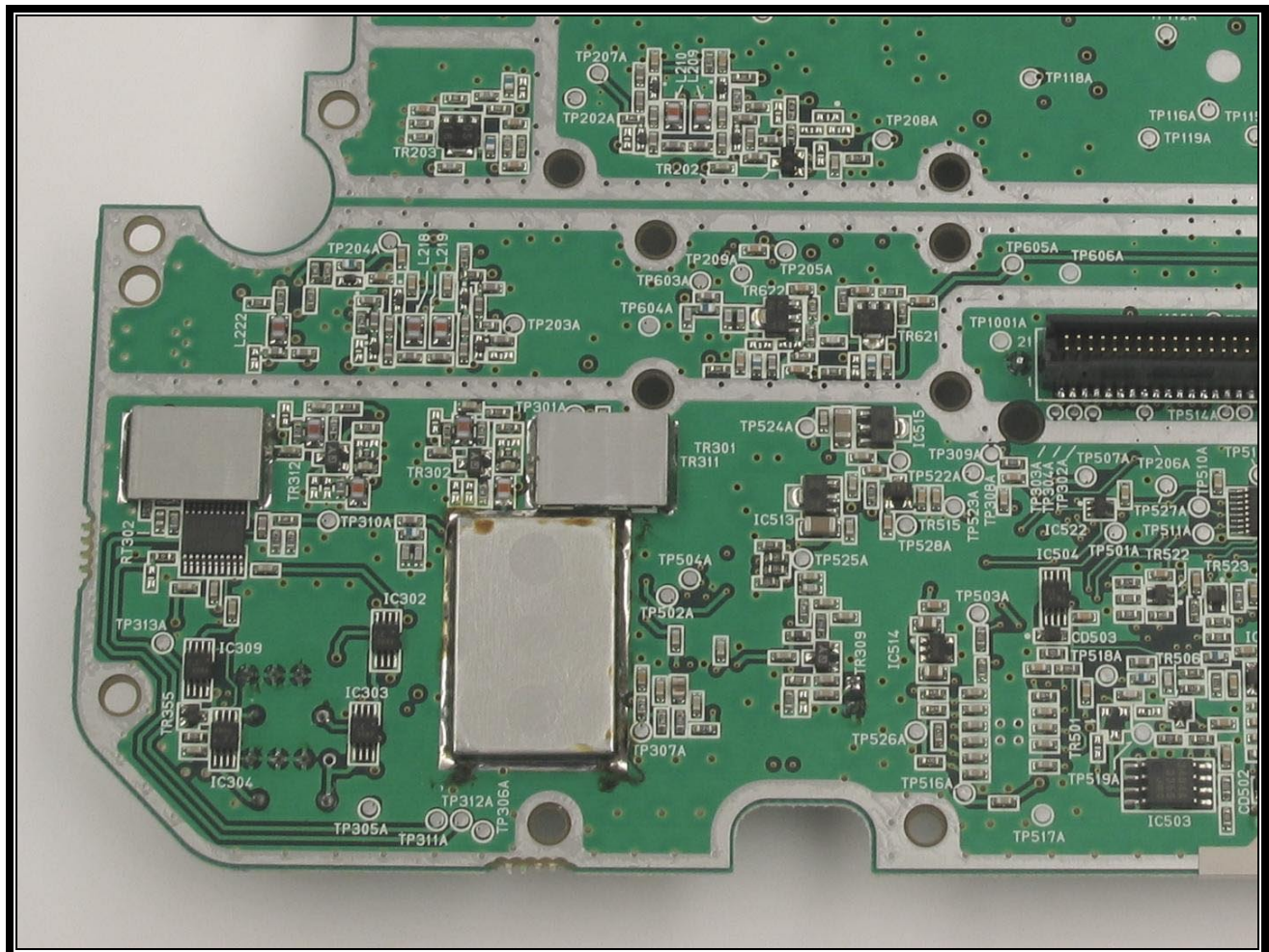
PHOTOGRAPH 24: TRX SYN BOARD SOLDER SIDE, LOWER LEFT
