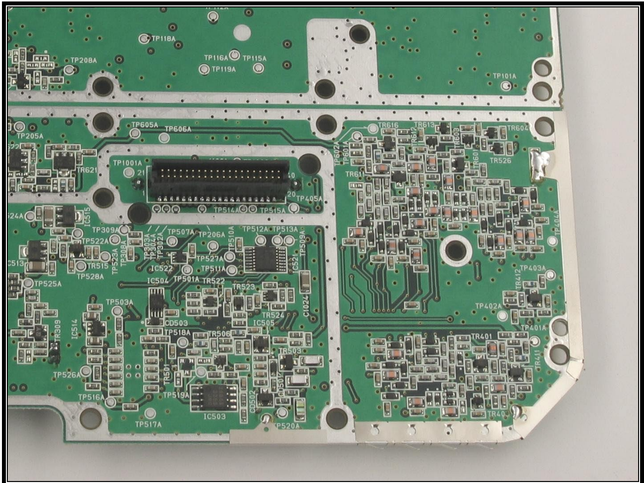
PHOTOGRAPH 25: TRX SYN BOARD SOLDER SIDE, LOWER RIGHT
