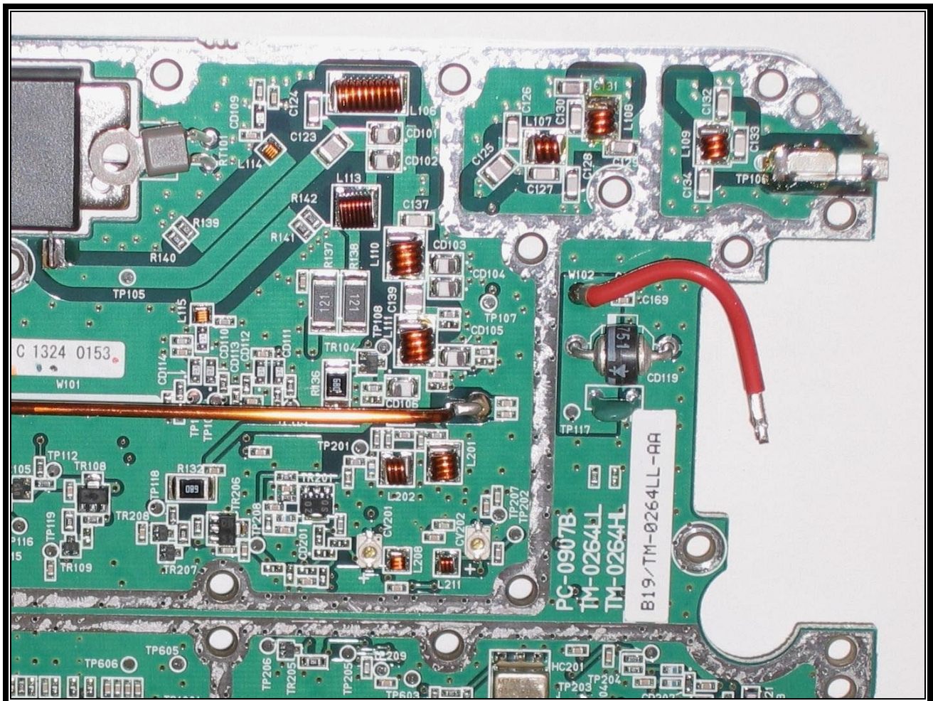
PHOTOGRAPH 22: TRX SYN BOARD COMPONENT SIDE, UPPER RIGH
