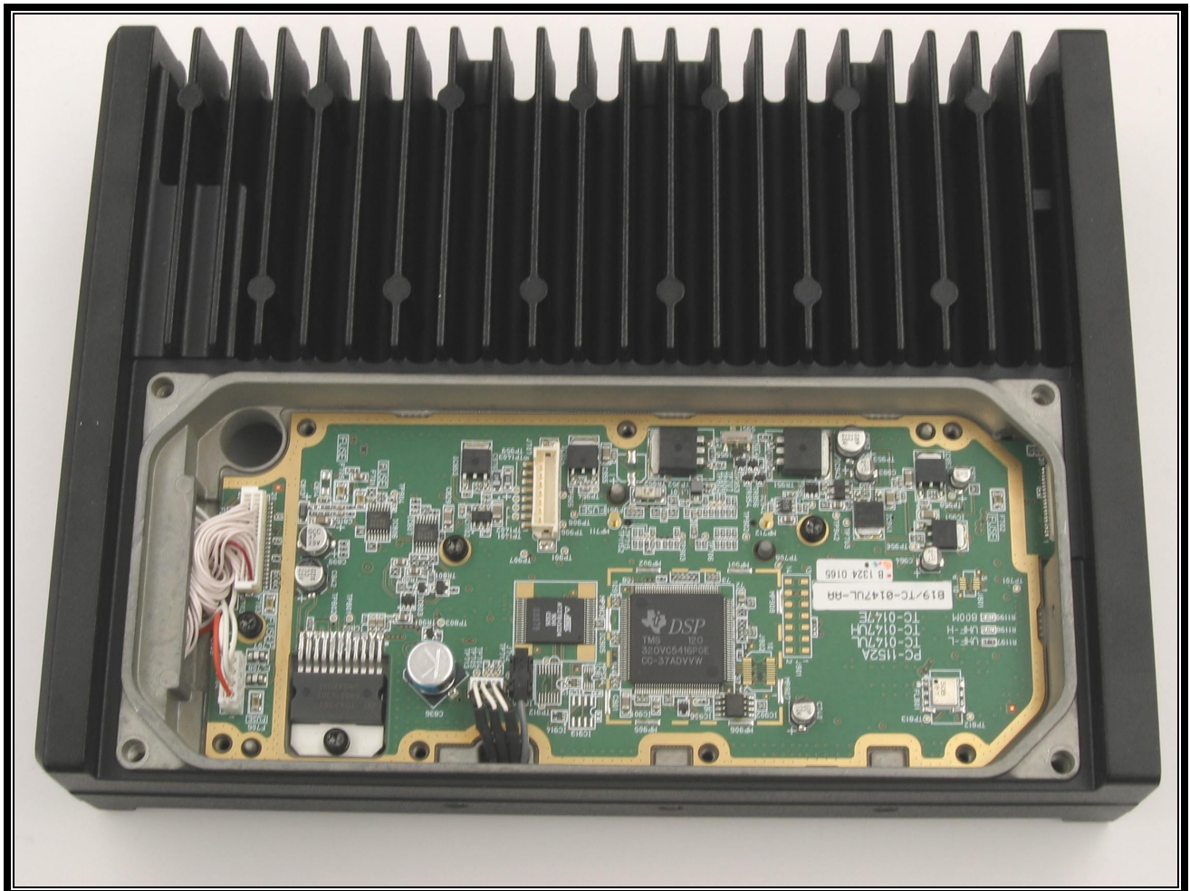
PHOTOGRAPH 17: TOP COVER AND INNER SHIELD REMOVED
