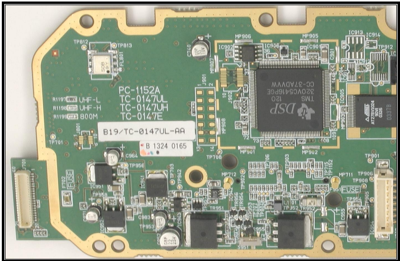
PHOTOGRAPH 12: AUDIO LOGIC COMPONENT SIDE, LEFT SIDE
