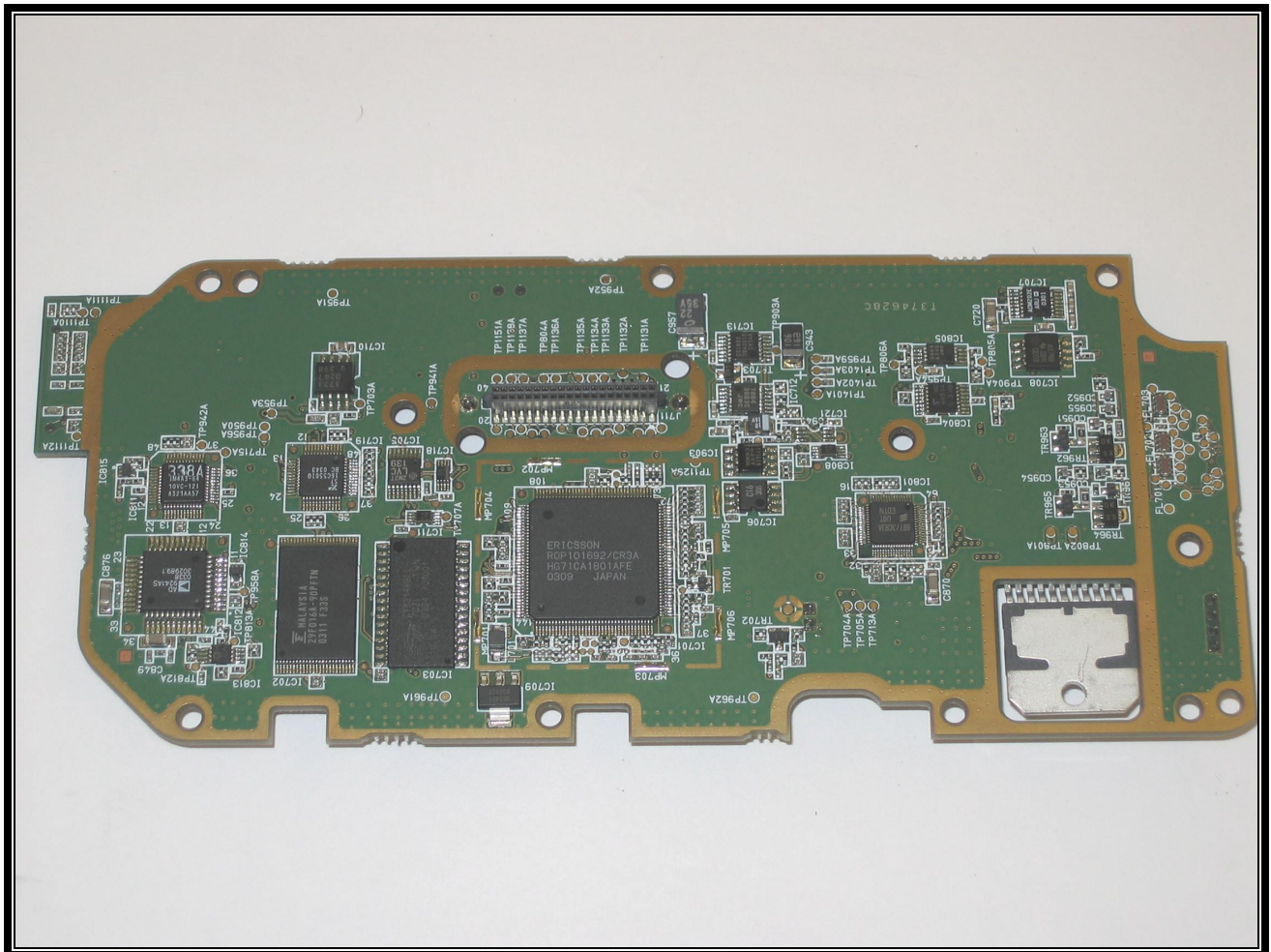
PHOTOGRAPH 14: AUDIO LOGIC BOARD SOLDER SIDE, COMPLETE VIEW
