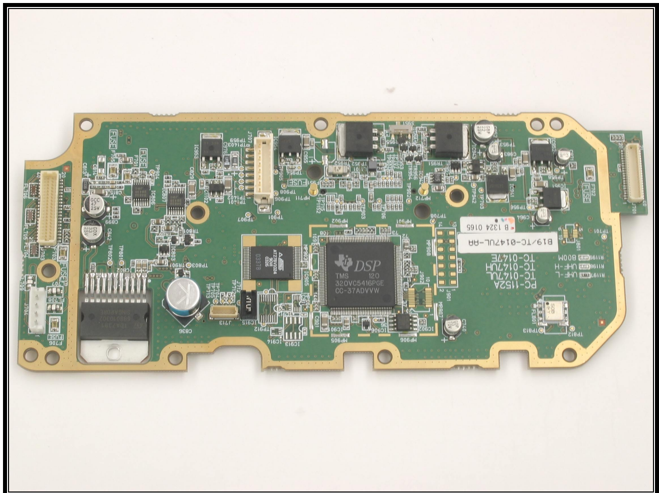
PHOTOGRAPH 11: AUDIO LOGIC BOARD COMPONENT SIDE, COMPLETE VIEW
