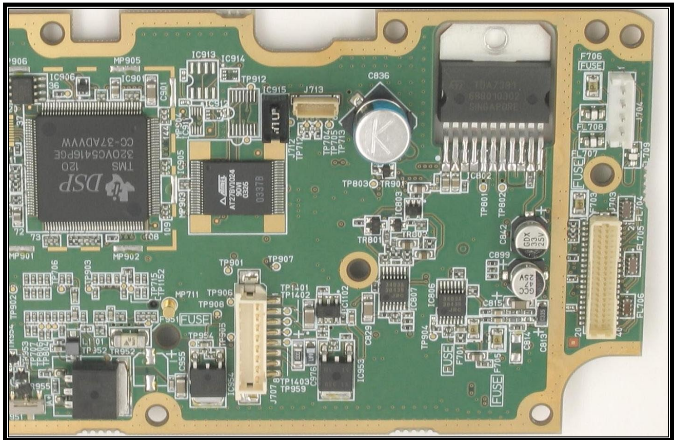
PHOTOGRAPH 13: AUDIO LOGIC COMPONENT SIDE, RIGHT SIDE
