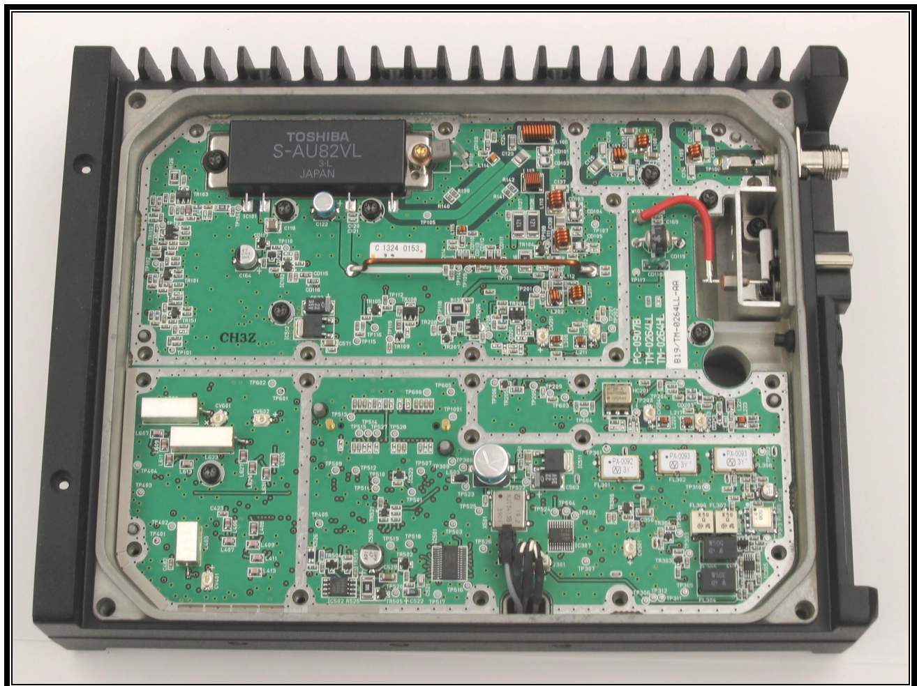
PHOTOGRAPH 10: BOTTOM COVER AND INNER SHIELD REMOVED
