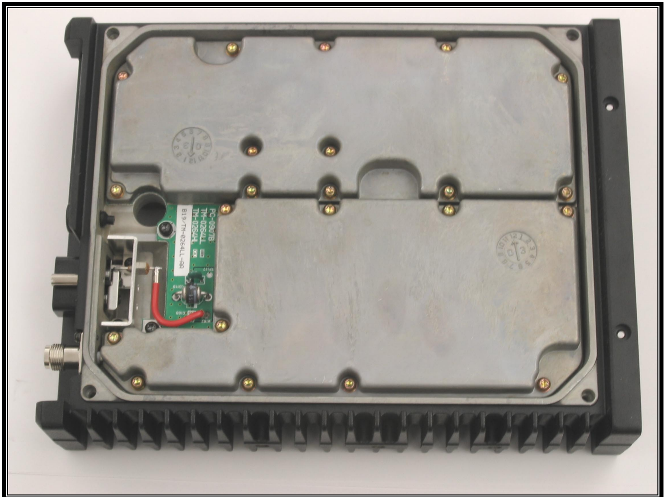
PHOTOGRAPH 9: BOTTOM COVER REMOVED
