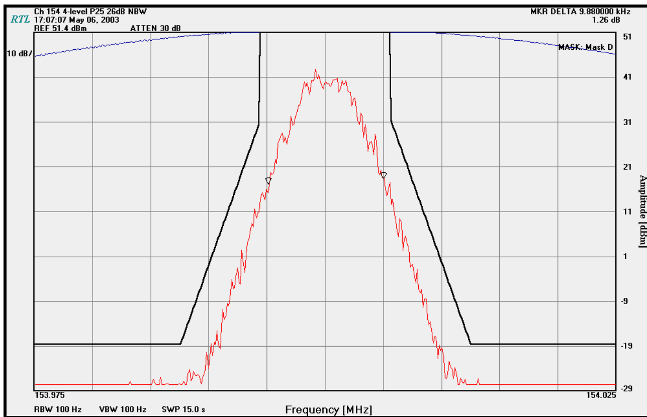
PLOT 14-3: 26 dB BANDWIDTH; NARROW BAND; C4FM DIGITAL MODULATION
