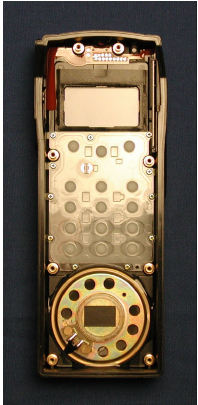
Rear Housing with Switch Module
