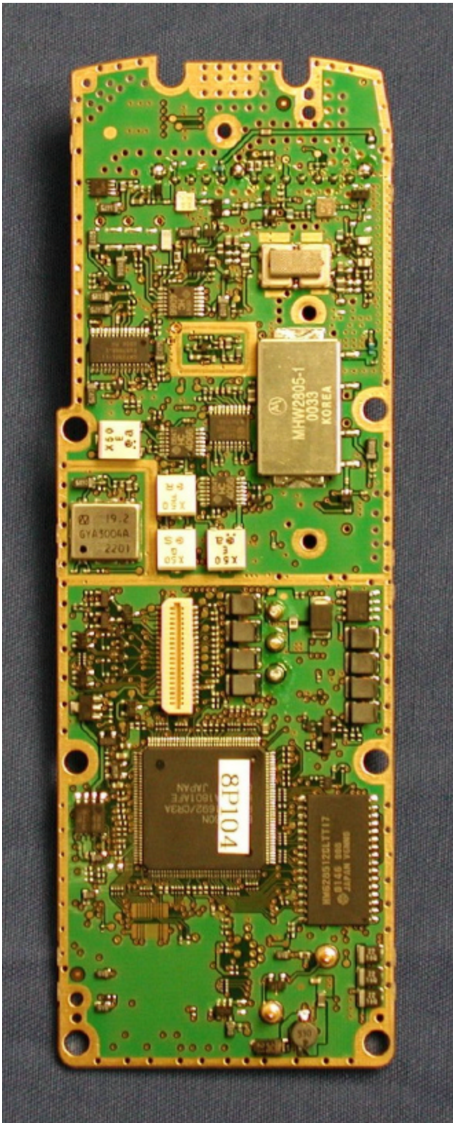
Main Board
