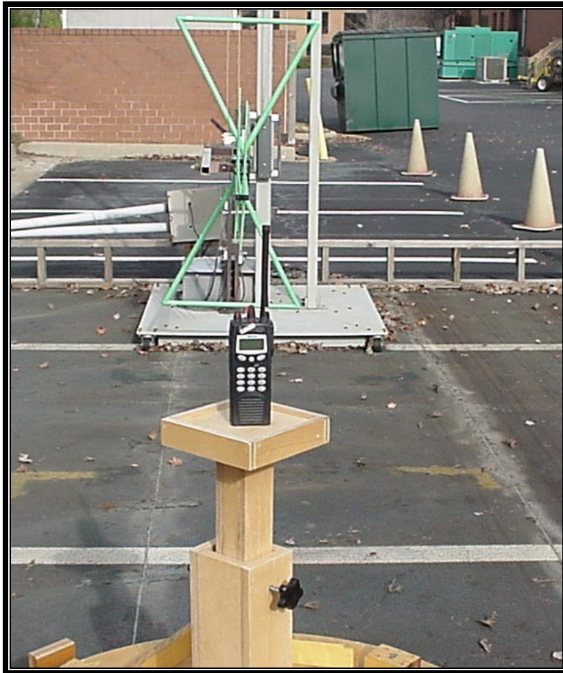
PHOTOGRAPH 1: RADIATED EMISSIONS FRONT VIEW
