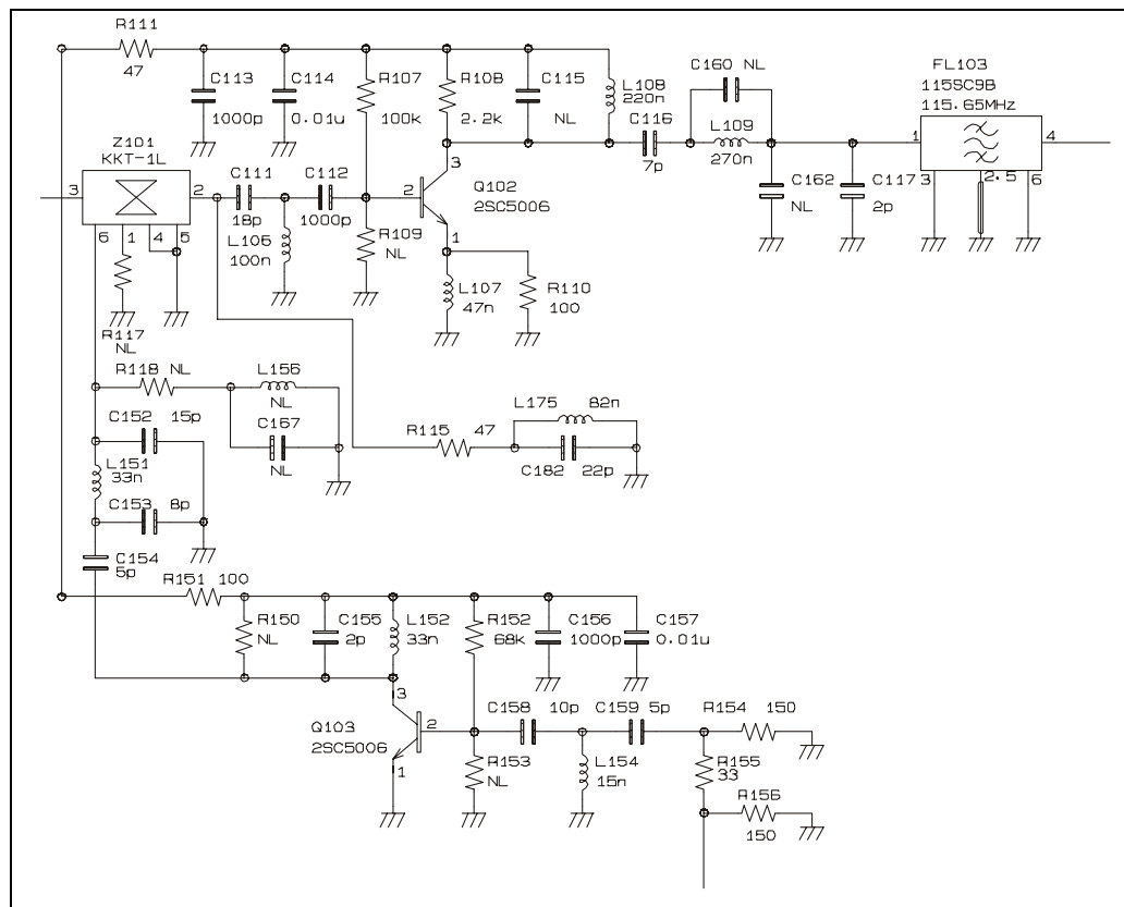
Figure 9 – UHF-H P7100 IP First Mixer and First I.F. Circuit Diagram
