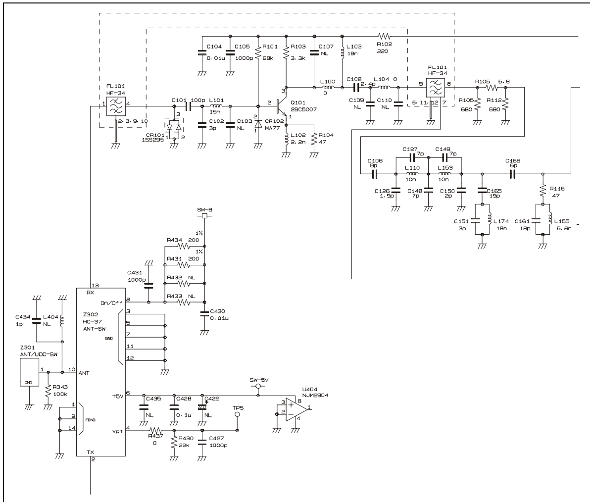
Figure 8 – UHF-H P7100 IP Receiver Bandpass Filter and Circuit Diagram
