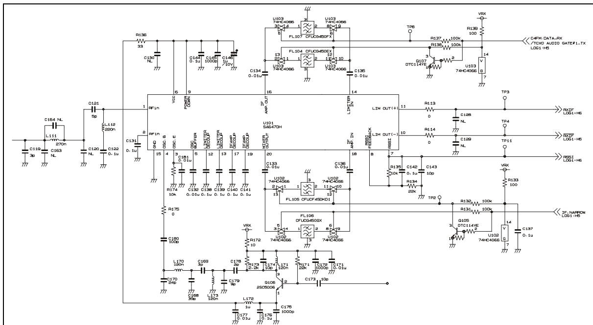
Figure 10 – UHF-H P7100 Second Mixer and Second IF Circuit Diagram
