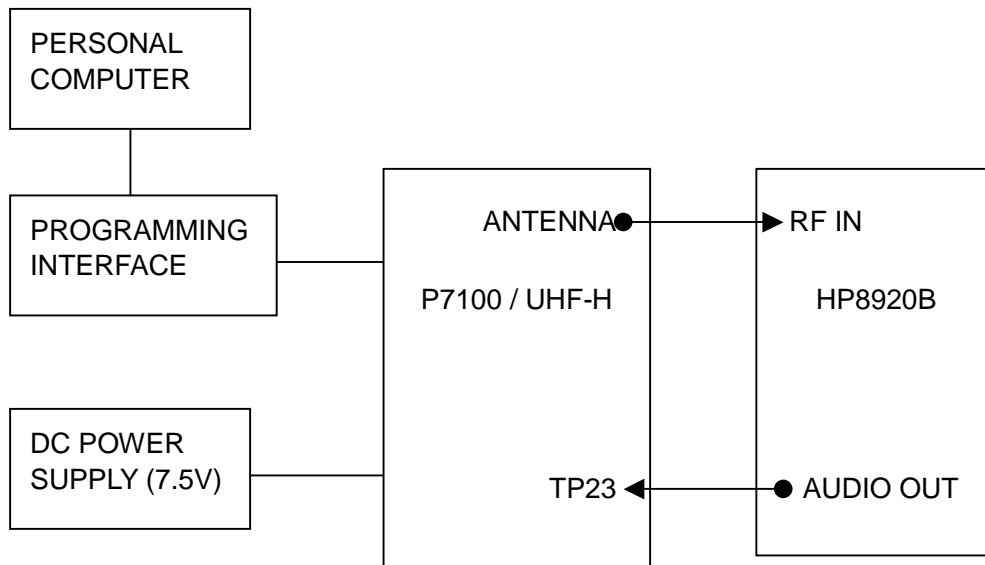
Figure 1: Equipment Setup
