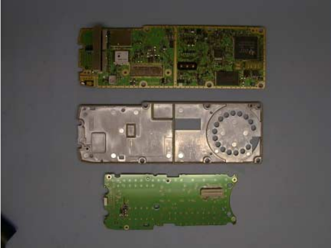
Internal PC Boards and Shield, Back
