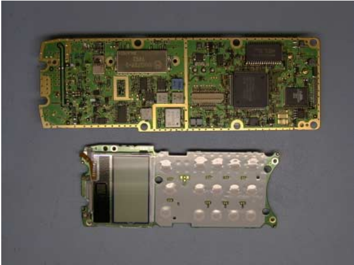
PC Boards, Front
