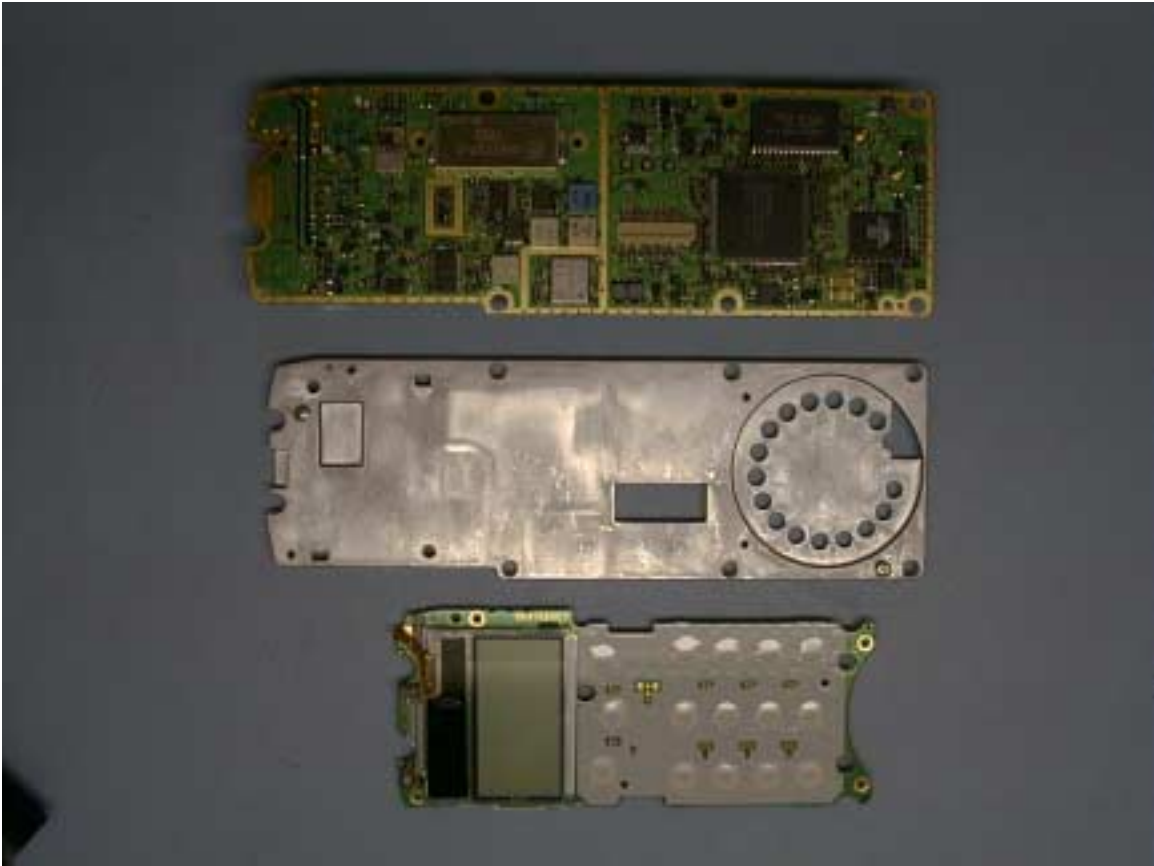
Internal PC Boards and Shield, Front
