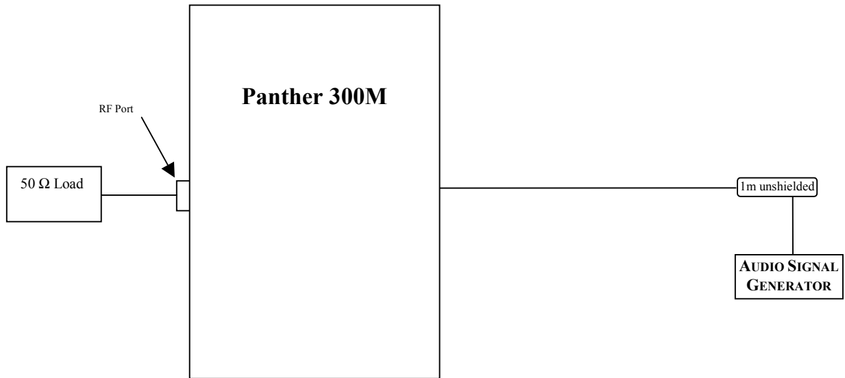
FIGURE 1: TEST CONFIGURATION
