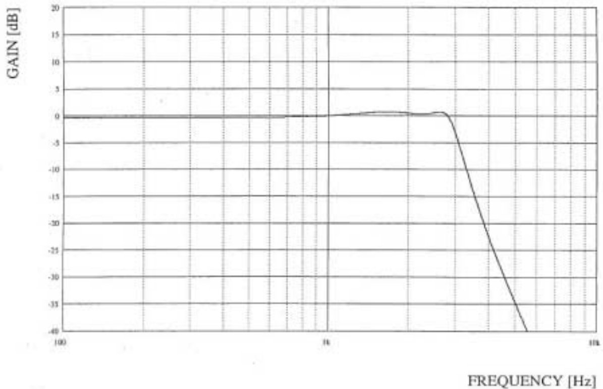
Fig.4.B LPF( F_c=2.55\text{kHz} ) Frequency Response (Reference)
