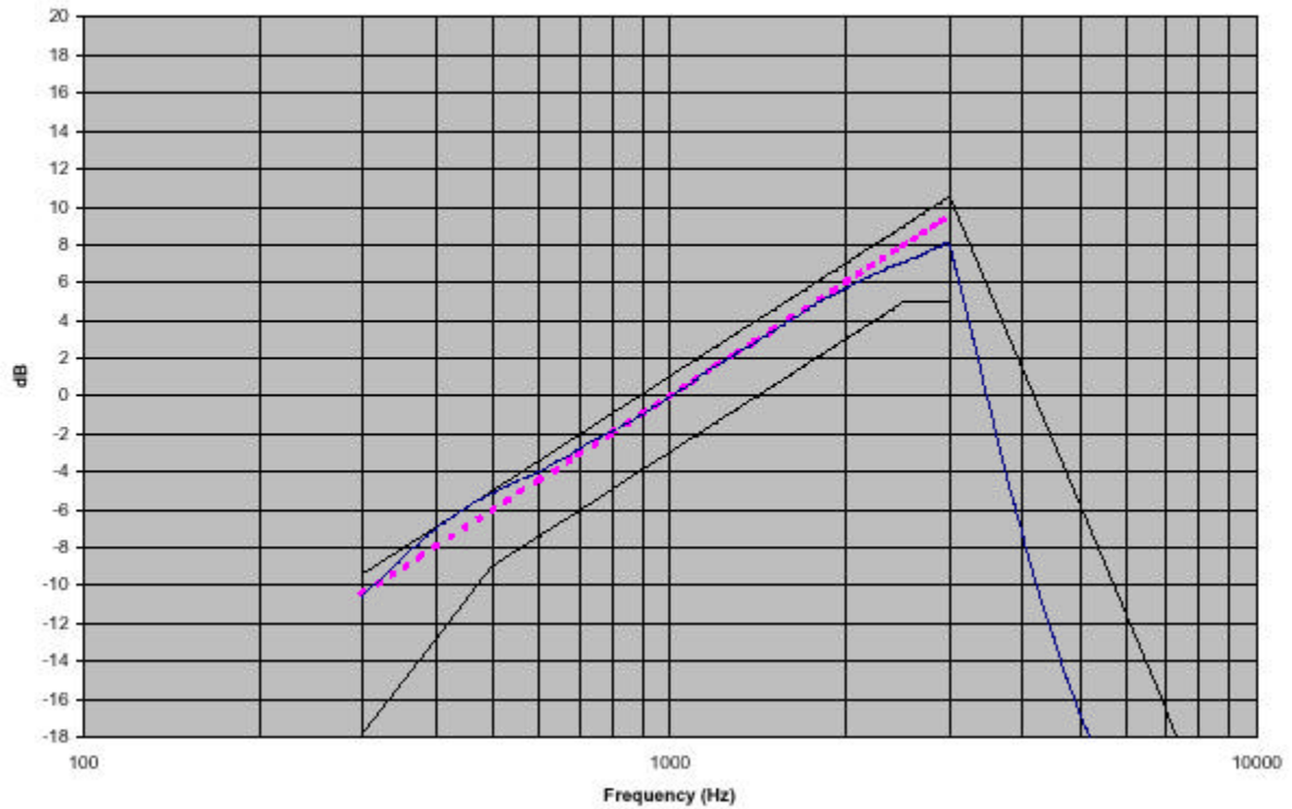
Channel 4 - 12.5 kHz Audio Frequency Response
