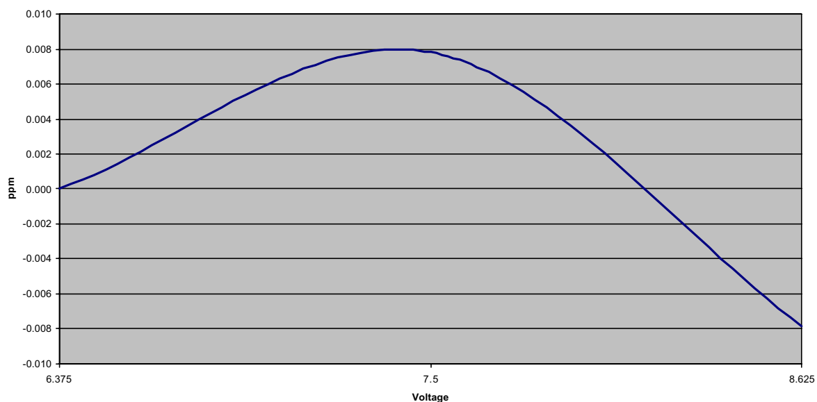
Voltage Frequency Stability (7.5 Nominal) Maximum deviation +/-0.008
