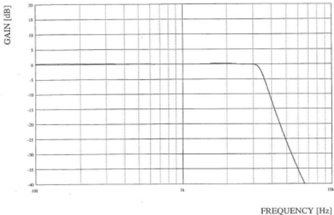
Fig.4.A LPF( F_c=3.0\text{kHz} ) Frequency Response (Reference)
