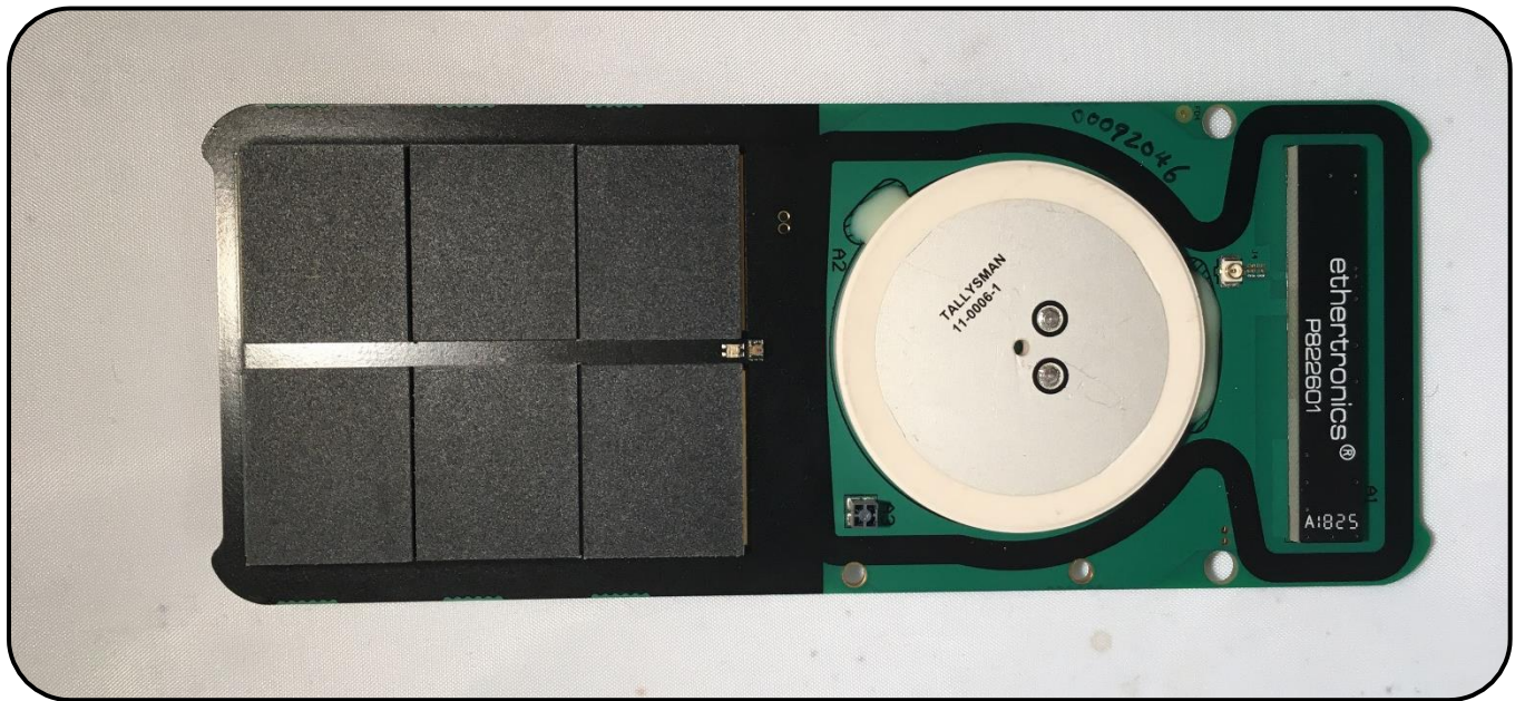
FIGURE 1: ANTENNA SIDE
