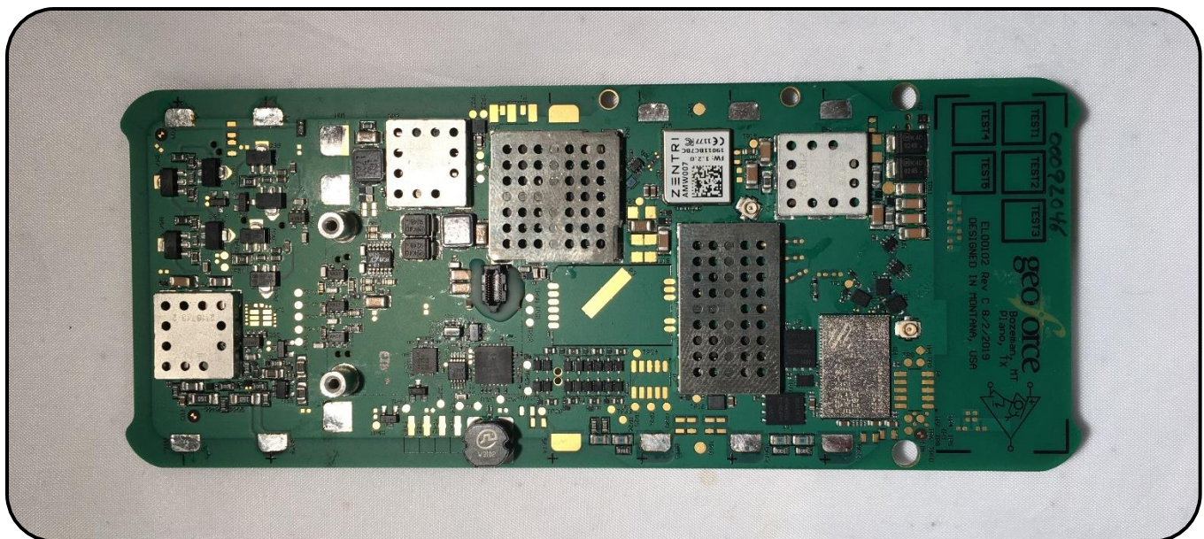
FIGURE 2: COMPONENT SIDE 1
