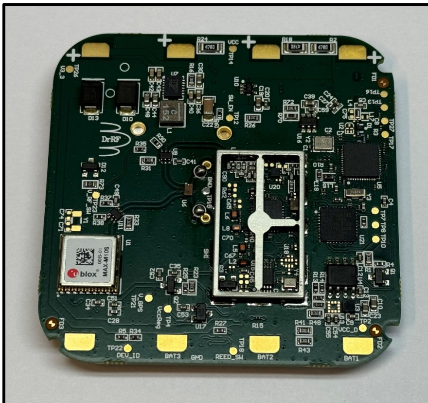
GT1/GT1s PCB Bottom, With Shield Rail
