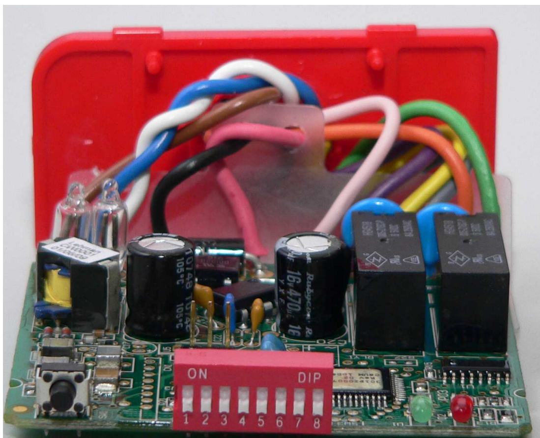
12/24V Models – Interior Front View
