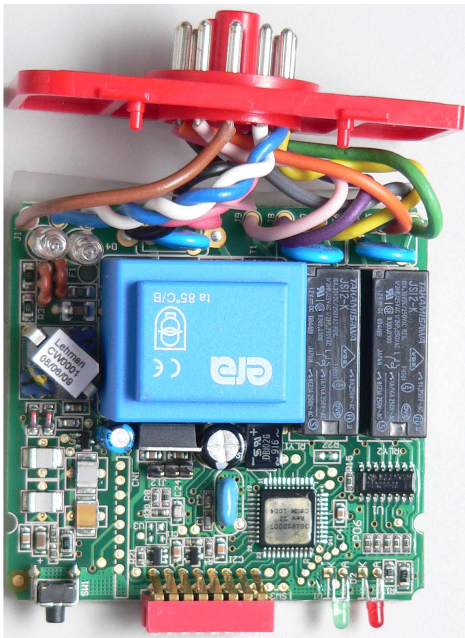
120 V & 230 V Models – Interior Top View
