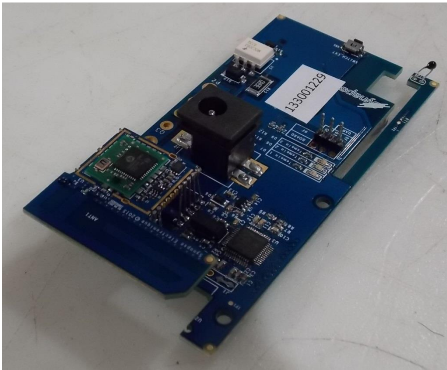
Figure 1-3: Side view – RF module on support PCB
