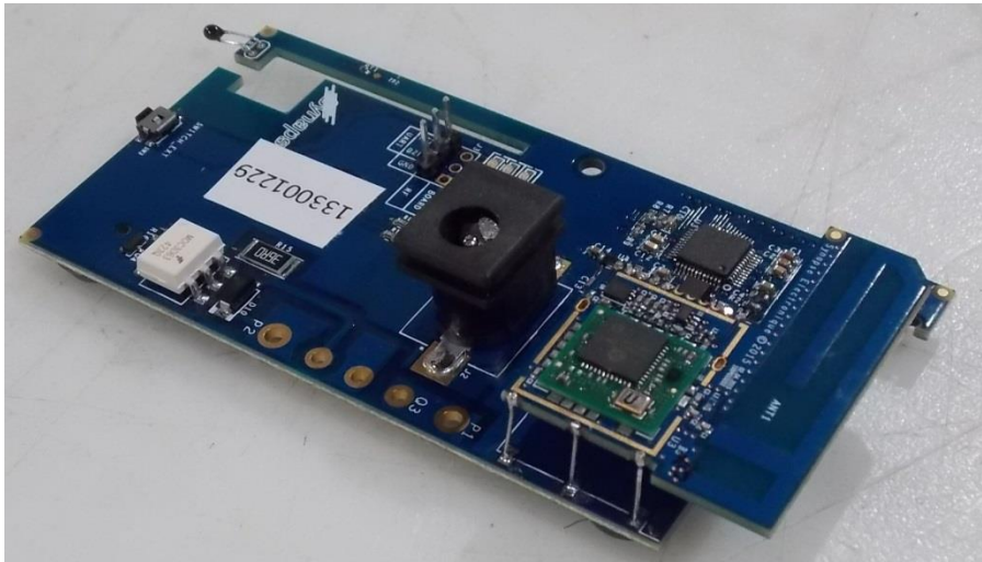
Figure 1-4: Side view – RF module on support PCB
