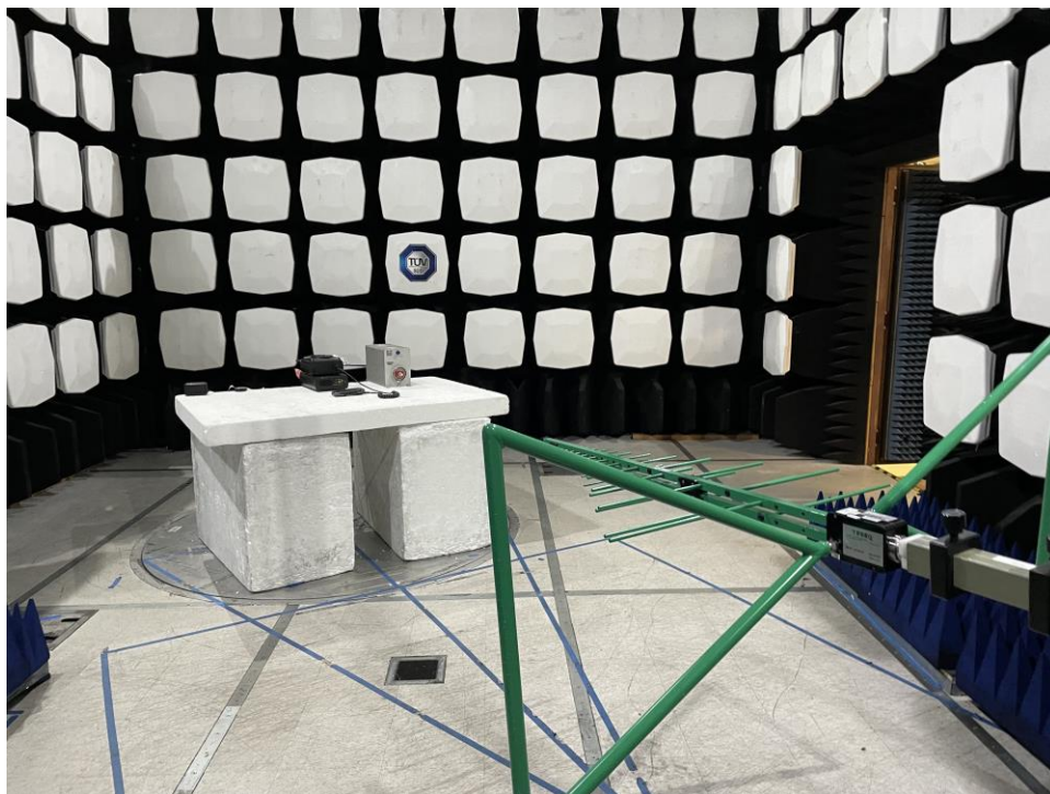
Figure A-3: Test Setup – Front View of the Radiated Emissions 30 – 500 MHz
