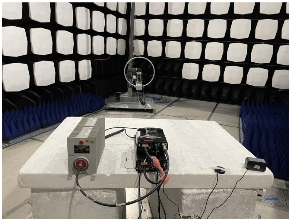
Figure A-2: Test Setup – Rear View of the Radiated Emissions 9kHz - 30 MHz
