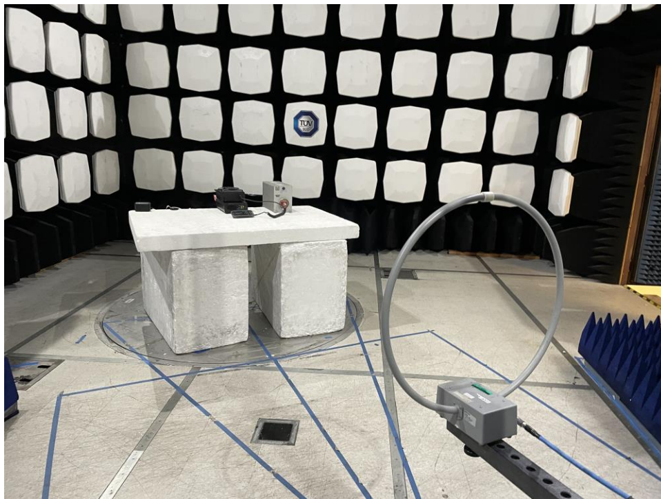
Figure A-1: Test Setup – Front View of the Radiated Emissions 9kHz - 30 MHz
