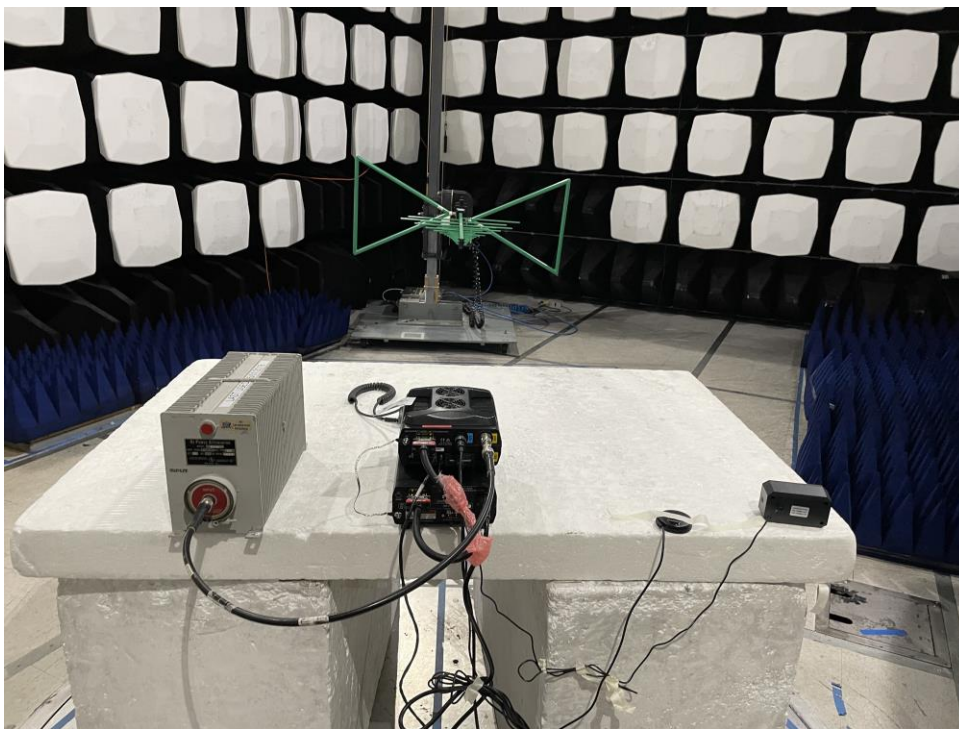
Figure A-4: Test Setup – Rear View of the Radiated Emissions 30 – 500 MHz
