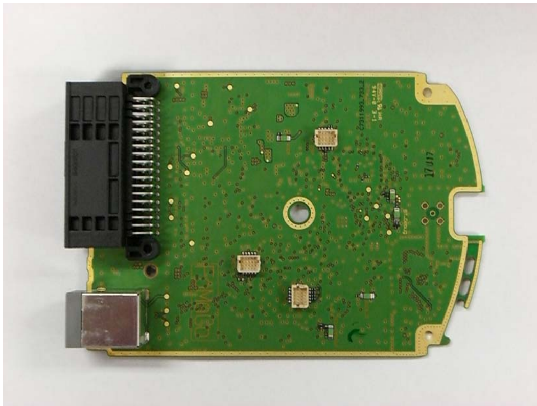
PWB to view
