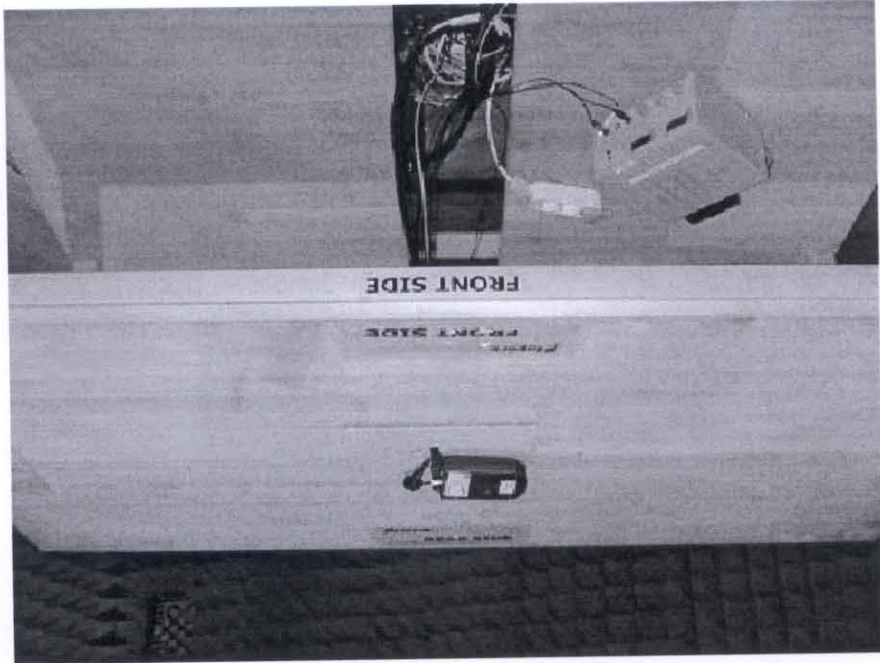
Picture 2 : Setup for the test "radiated emission"
