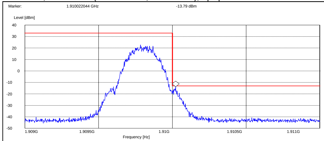
GSM mode, channel 810 (Peak detector, RBW: 3 kHz), flip open
