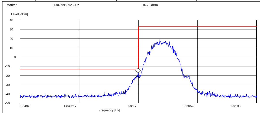
GSM mode, channel 512 / 1850.2 MHz (Peak detector, RBW: 3 kHz)
