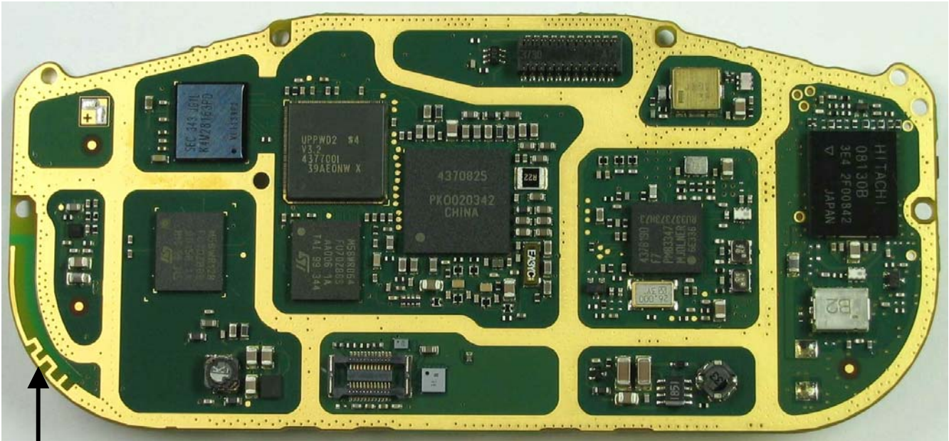
Bluetooth Antenna
