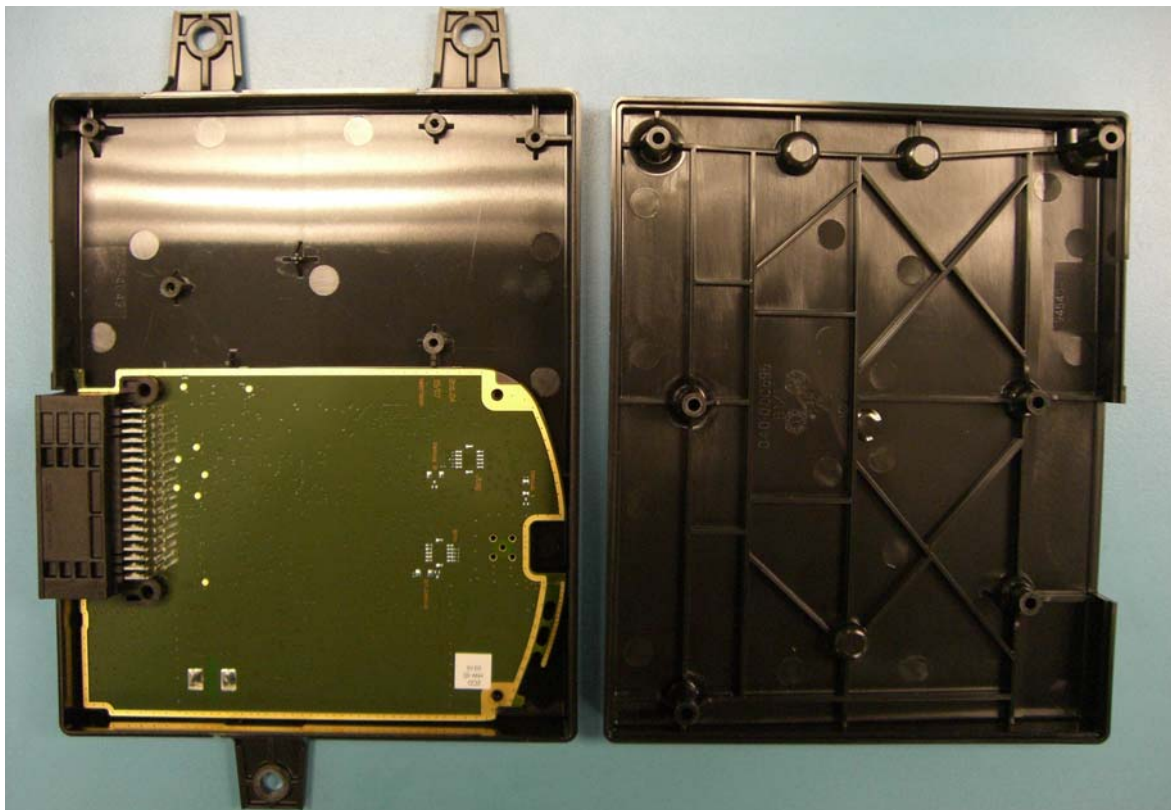
Mechanic with PWB bottom view
