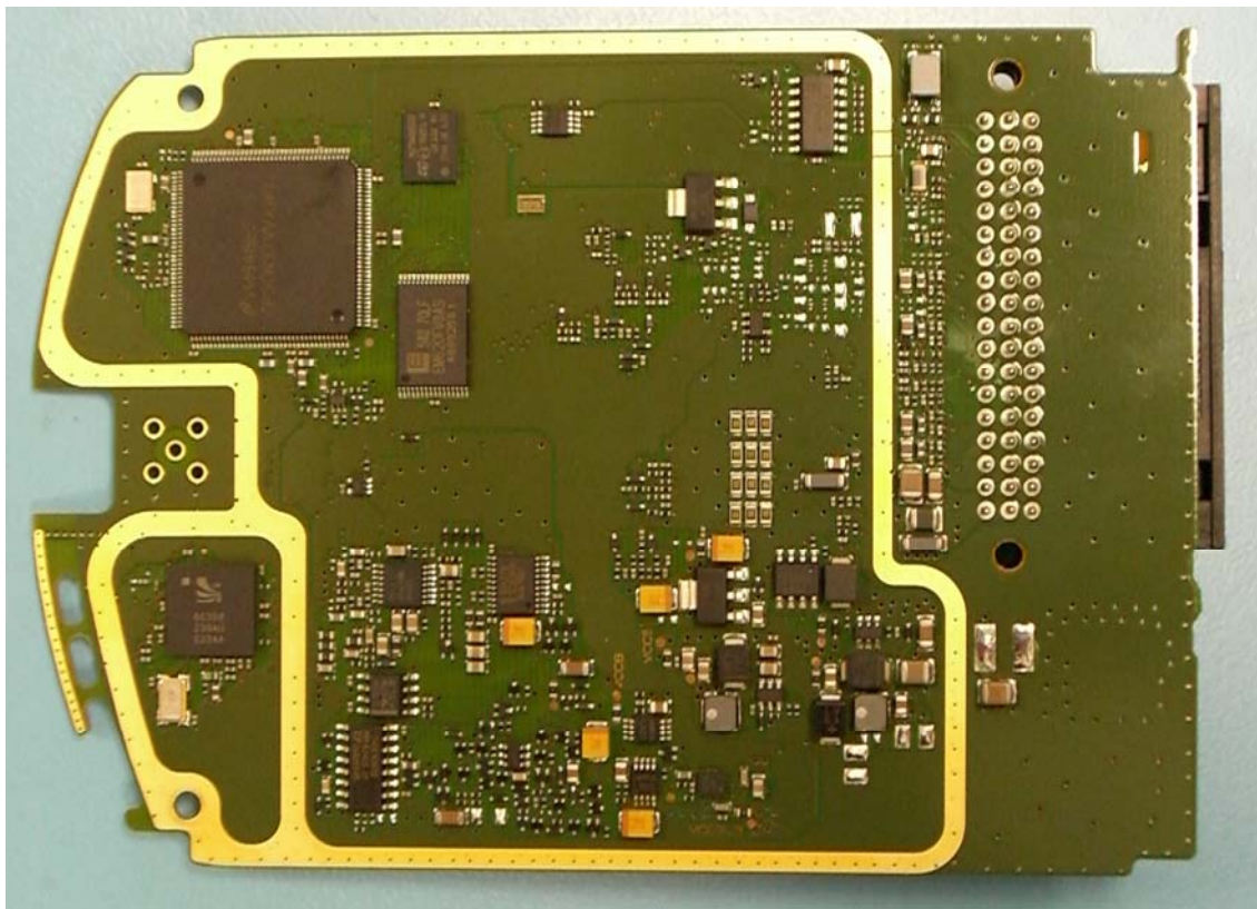
PWB bottom view with connector
