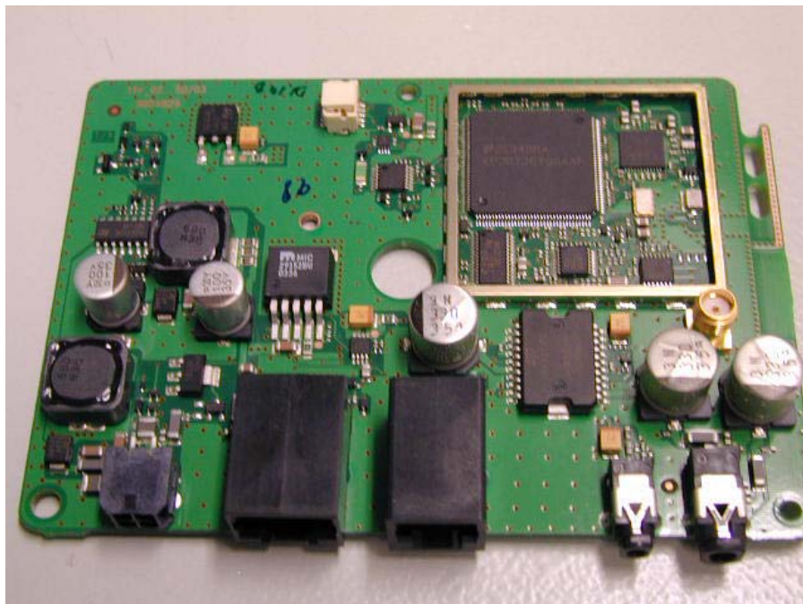
HF-5 front (shielding open) (EUT for conducted measurements)
