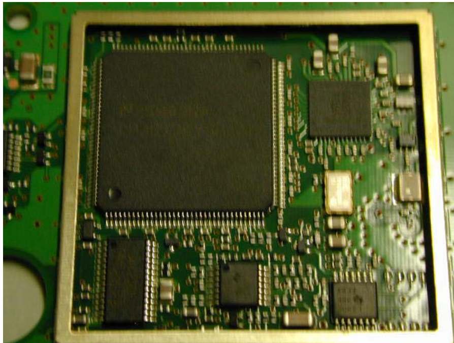
HF-5 front (RF) (EUT for conducted measurements)
