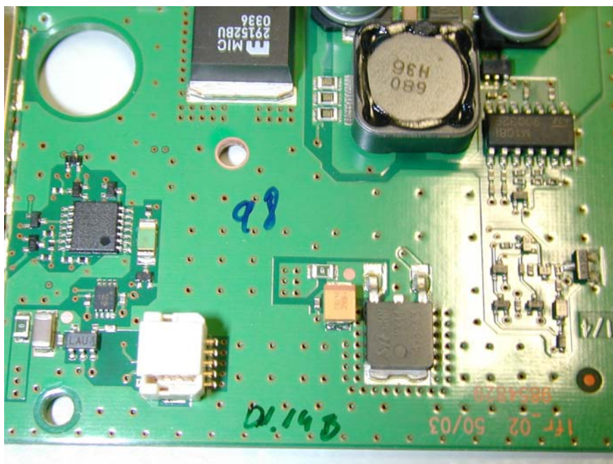
HF-5 front (Sample No. 98) (EUT for conducted measurements)
