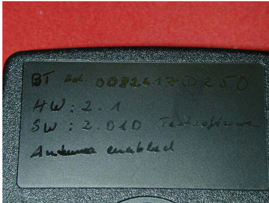
HF-5 back (EUT for conducted measurements)
