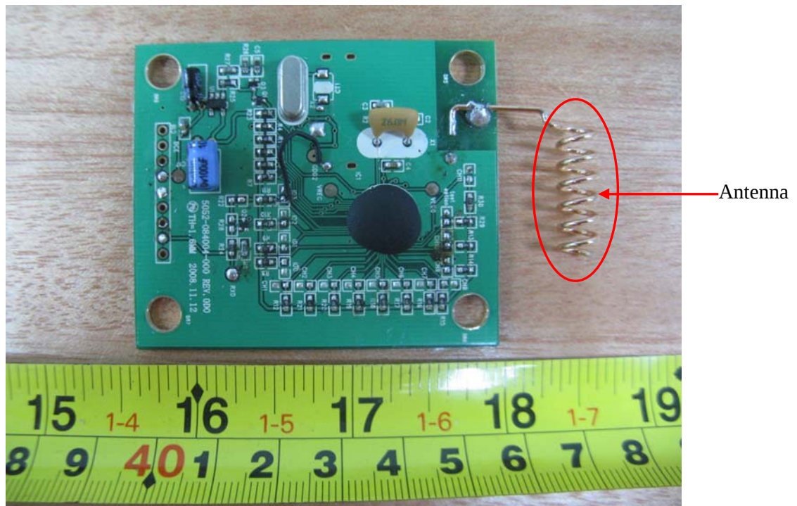
EUT - RF Board Top Components View
