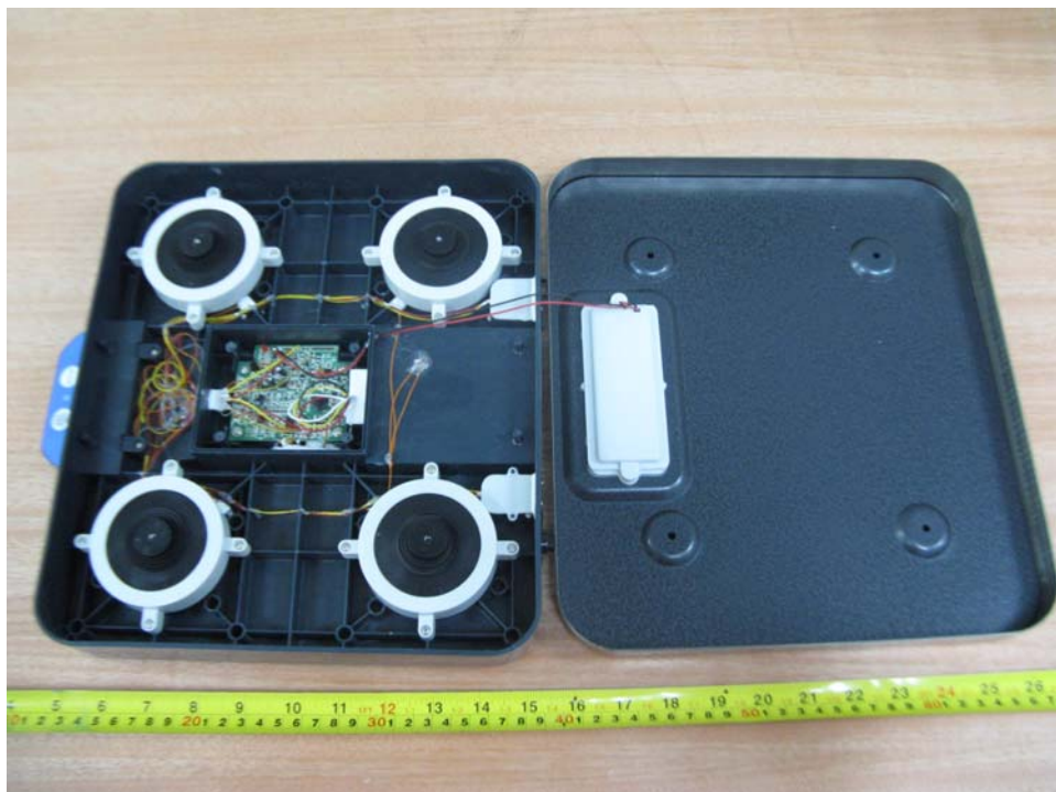
EUT – Main Module Uncovered View
