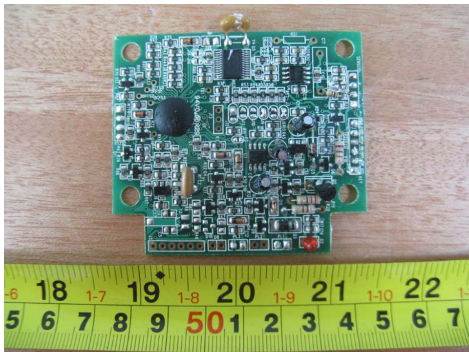
EUT - Mainboard Top Components View
