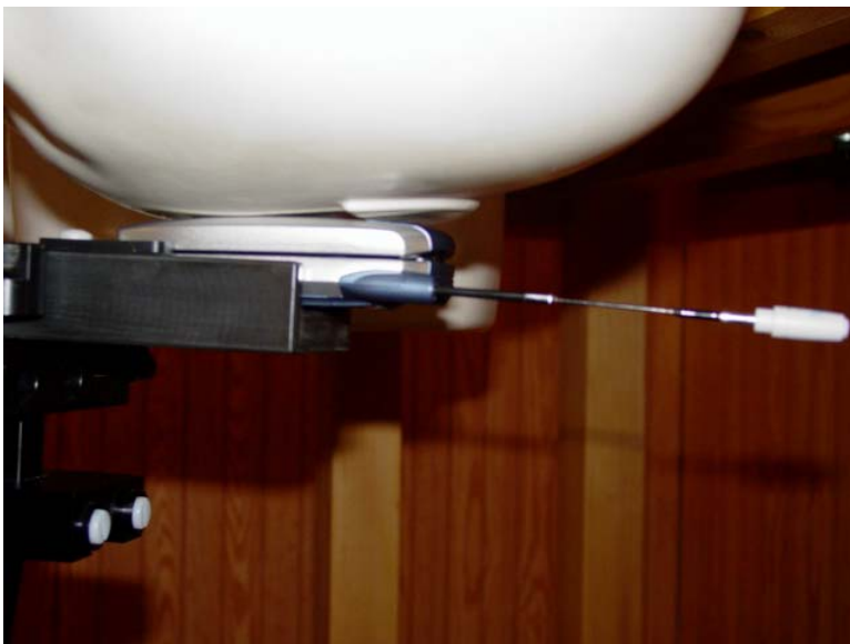
Figure 10.4 phone against the head (right cheek position, swivel closed, antenna extended)
