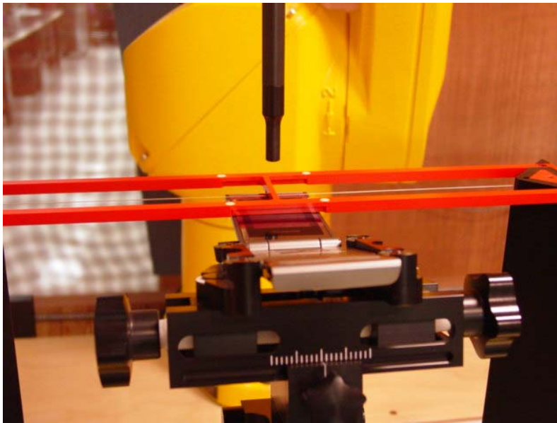
Figure 1a – HAC RF Emission Test Setup
