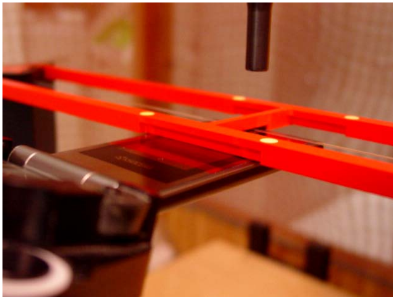
Figure 1b – HAC RF Emission Test Setup
