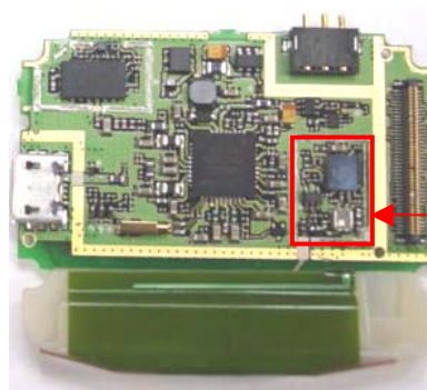
Bluetooth Circuitry
