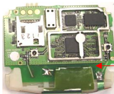
Bluetooth Antenna
