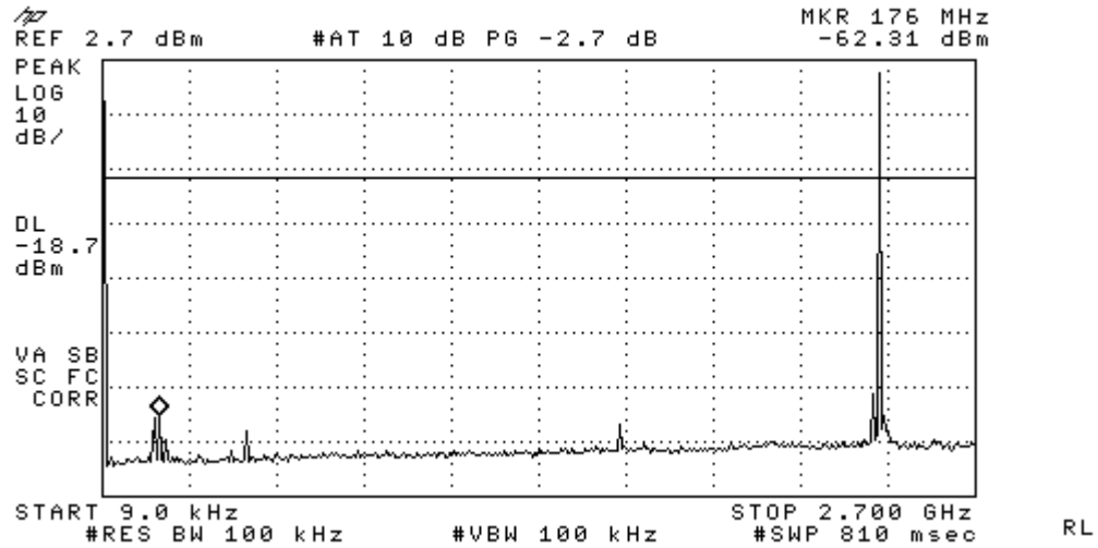
Figure 9-1a. Conducted Spurious Emissions (CH 0)
