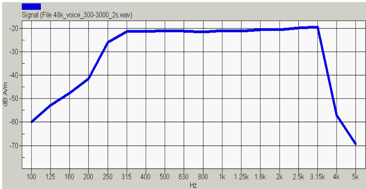
Figure 7.2b Broadband signal spectrum
