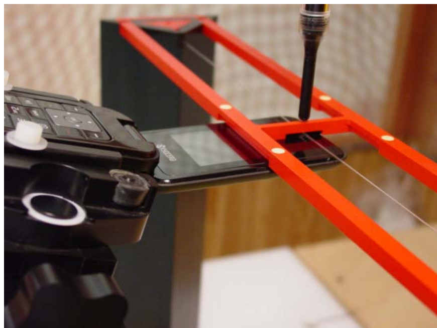
Figure 1b – HAC RF Emission Test Setup
