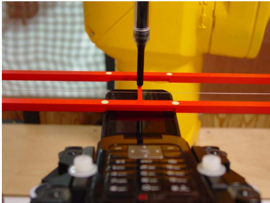
Figure 1a – HAC RF Emission Test Setup
