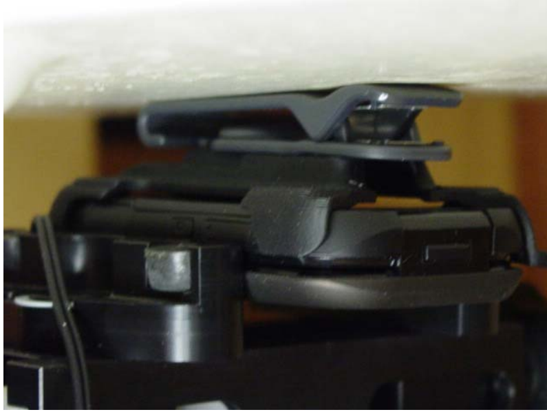
Figure 9E.6 Body SAR Phone setup Flip Closed with Holster (CV90-R2091-01)
