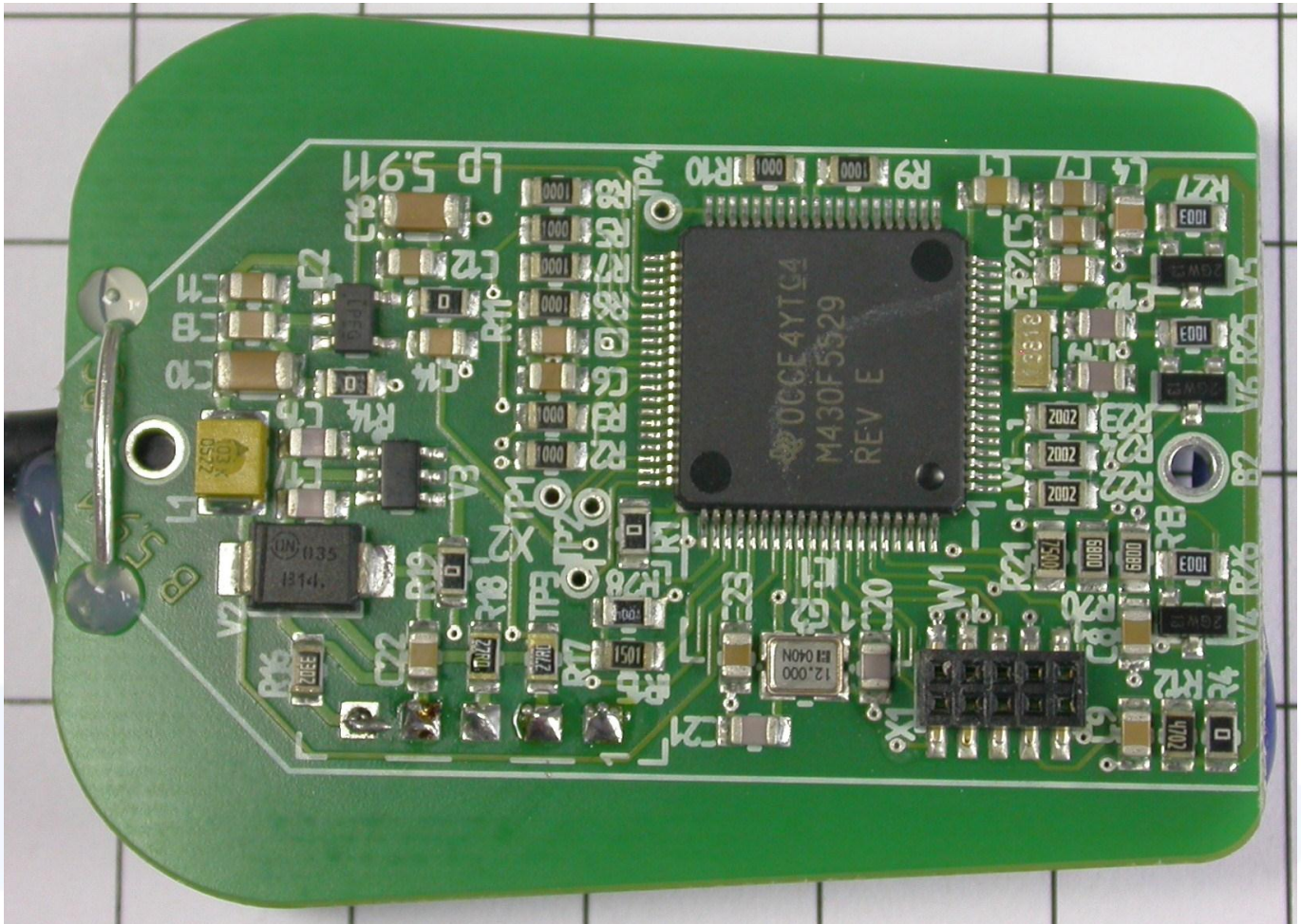
PCB bottom view
