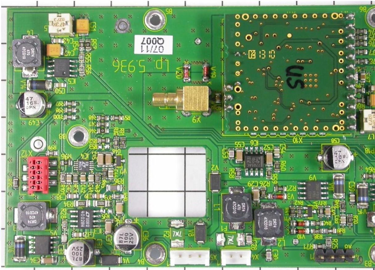
PCB top view (zoom)
