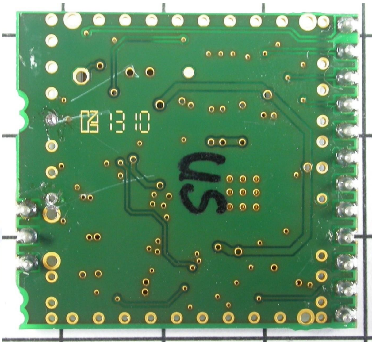
Top view – RF module
