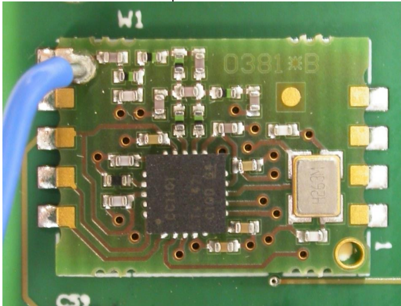
PCB Top view of RF modul
