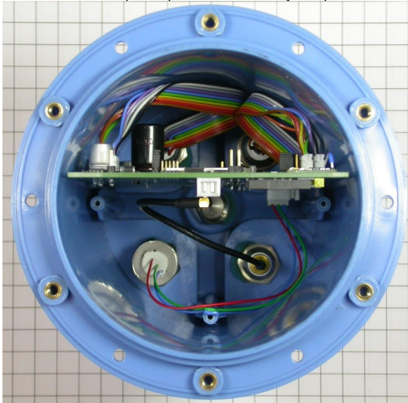
EuT top view (with removed battery case)
