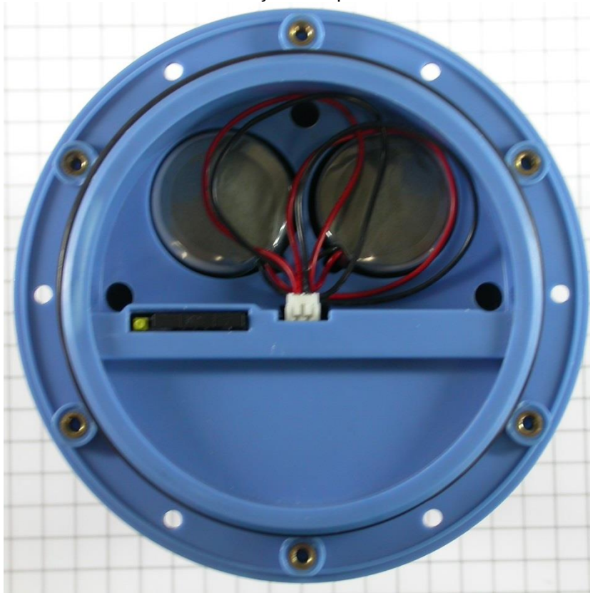
EuT top view (with removed front cover) Battery case top view
