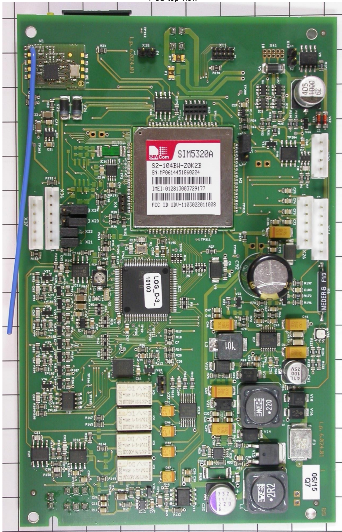
PCB top view
