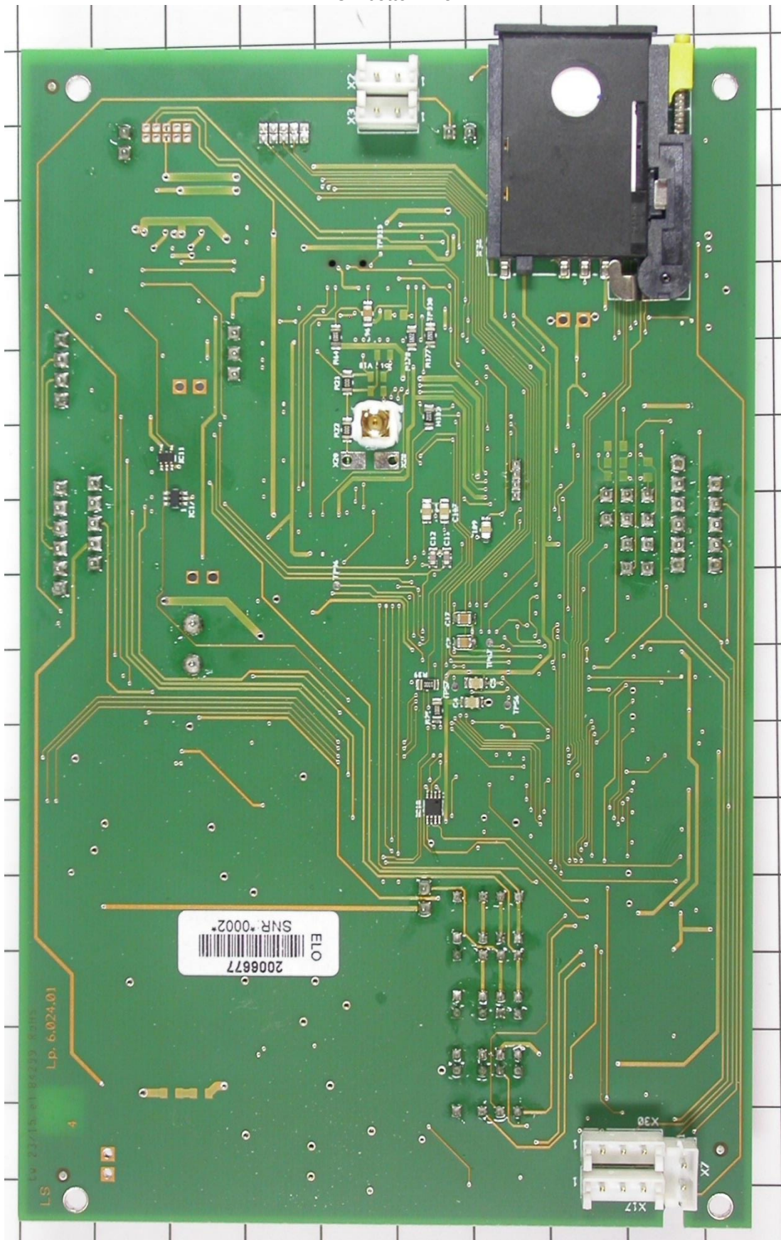
PCB bottom view
