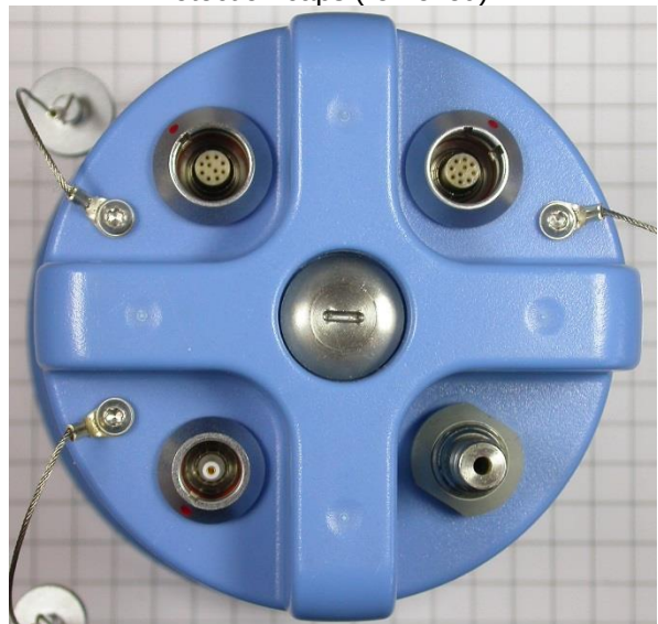
Protection caps (removed)
