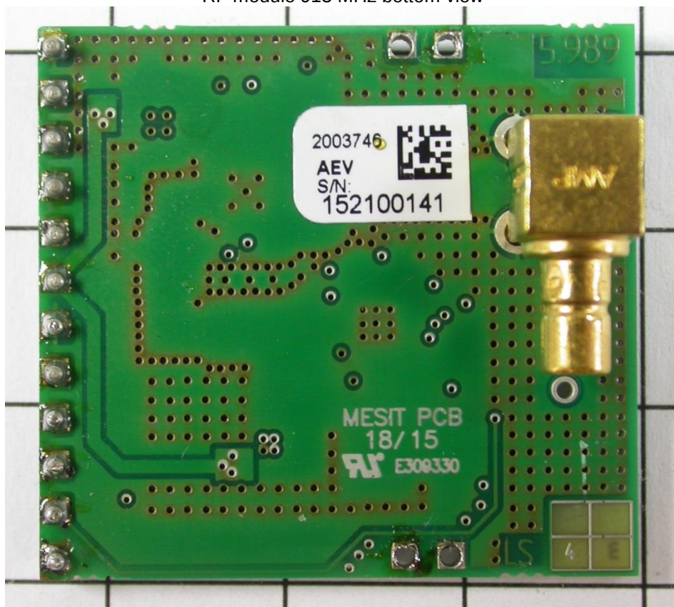
RF module 913 MHz bottom view
