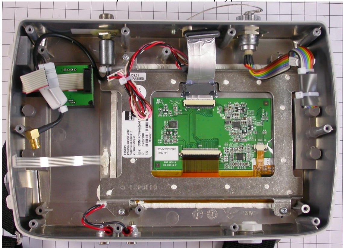
Front panel / connector view / display panel
