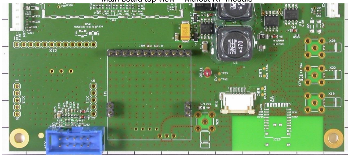
Main board top view – without RF module
