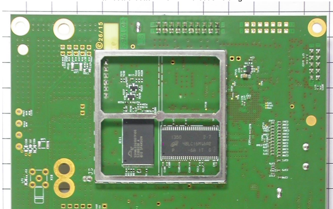
Mainboard bottom view – without shielding
