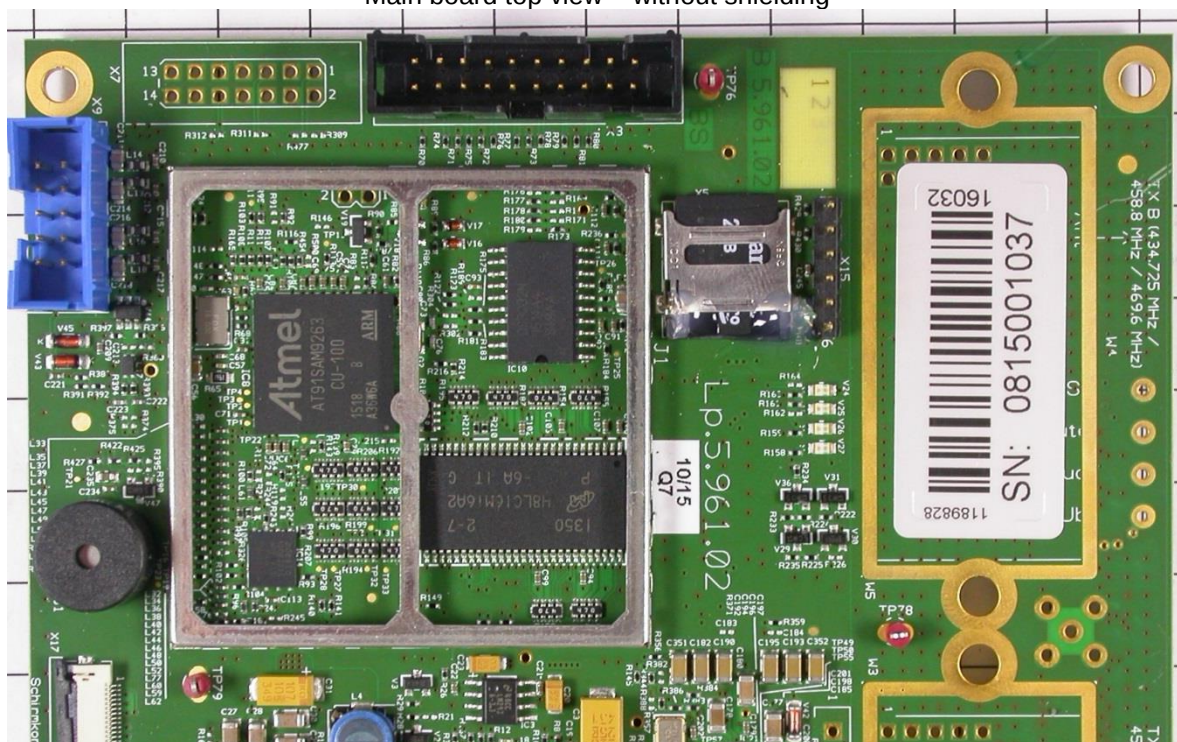
Main board top view – without shielding
