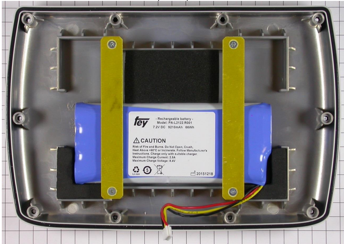
Front panel top view
