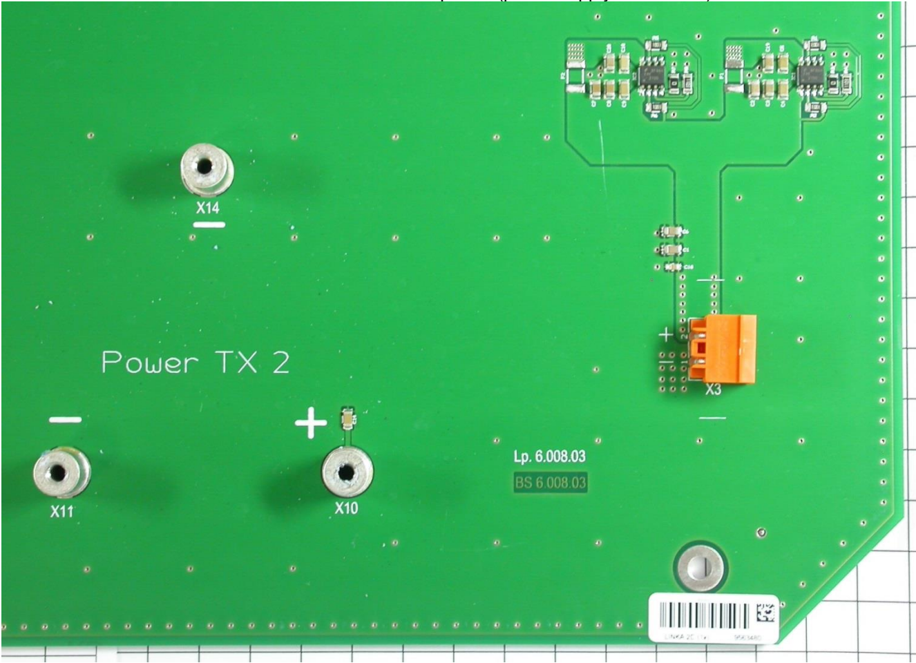
PCB mainboard – detailed top view (power supply connection)
