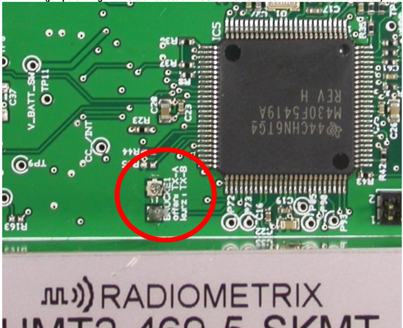
Mainboard detailed top view (jumper / bridge for version selection "COR PT-3A-913-469" or "COR PT-3B-913-469")
