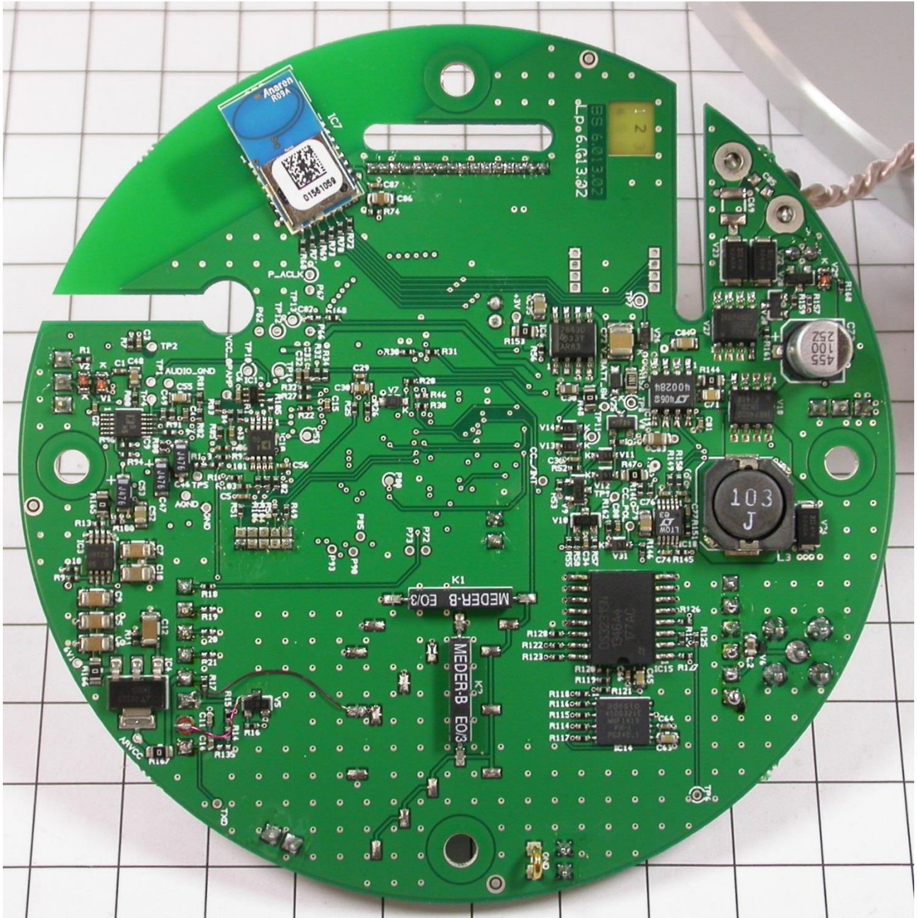
Mainboard bottom view
