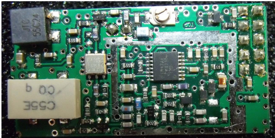
RF receiver modul 469 MHz top view
