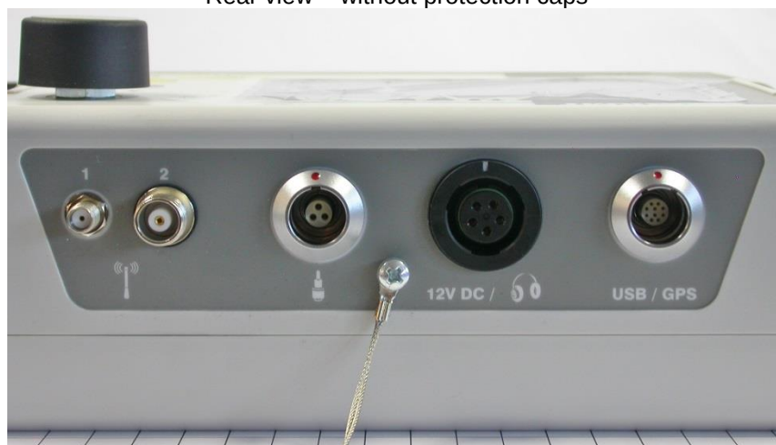
Rear view – without protection caps
