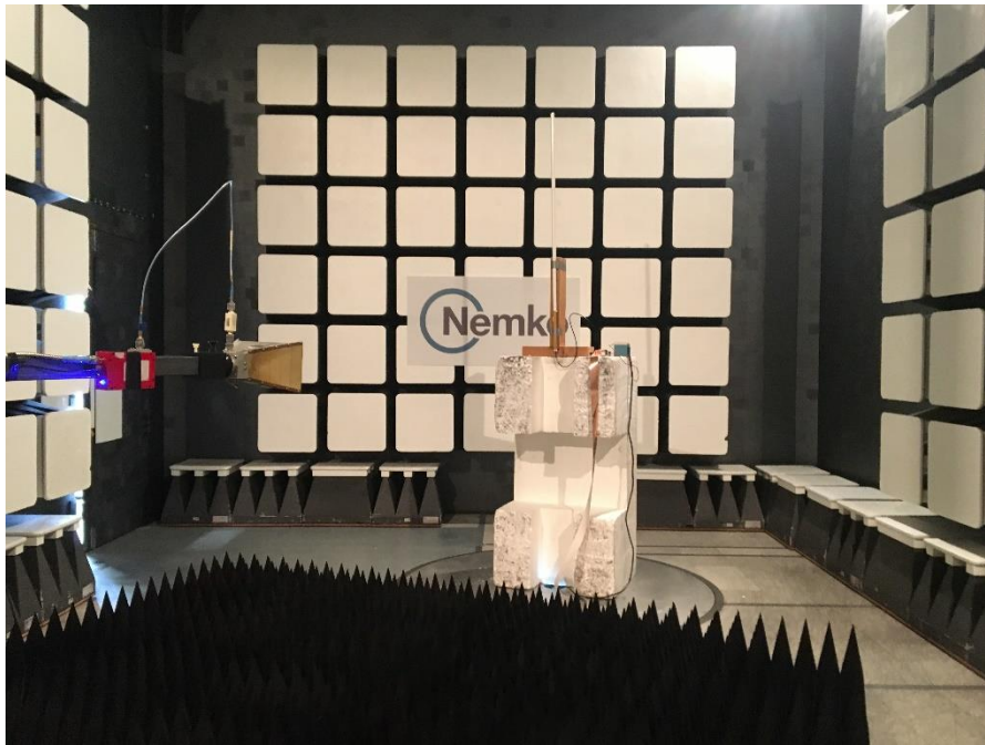
Figure 1.1-6: Radiated emissions setup photo – above 1 GHz (Rod Antenna, MN: FG9026)
