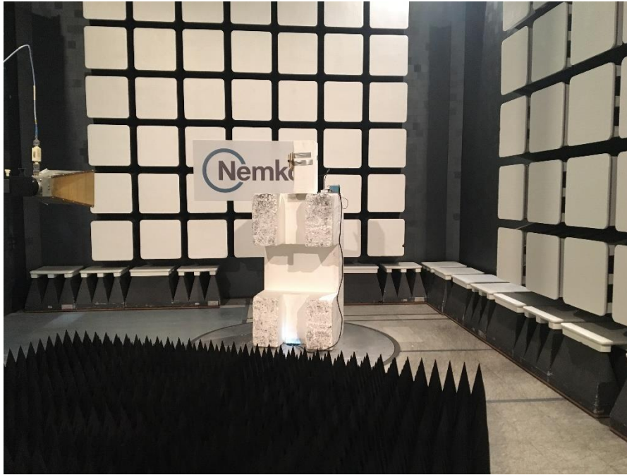
Figure 1.1-7: Radiated emissions setup photo – above 1 GHz (Yagi antenna, MN: Y8963)
