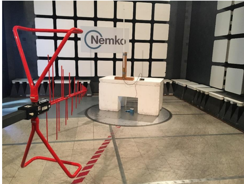
Figure 1.1-1: Radiated emissions setup photo – below 1 GHz (Rod Antenna, MN: FG9026)
