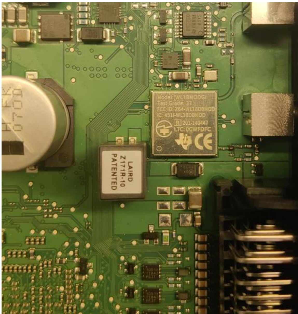
Wi-Fi PCB Close Up
