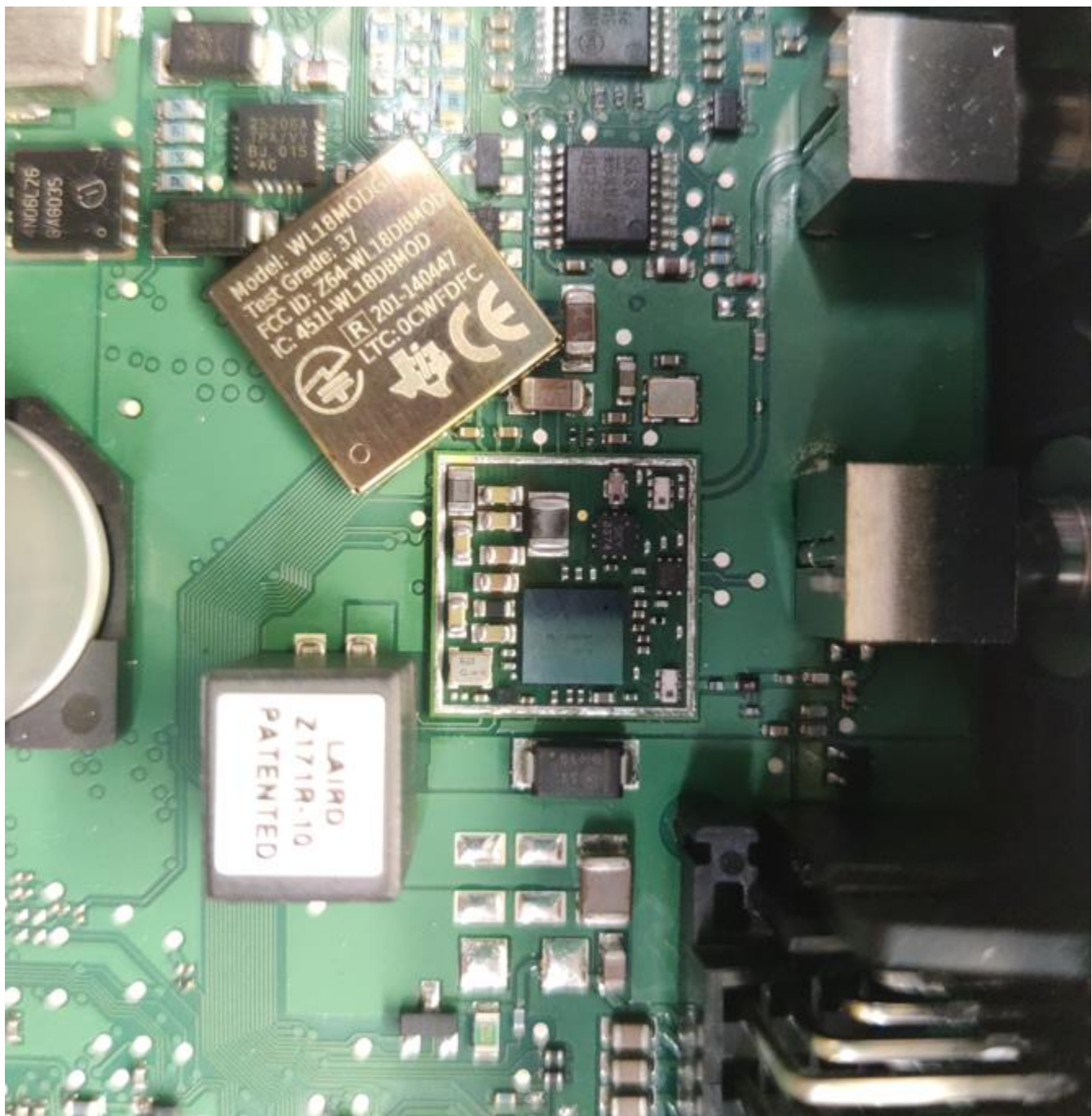
Wi-Fi PCB Close Up – Shield Removed
