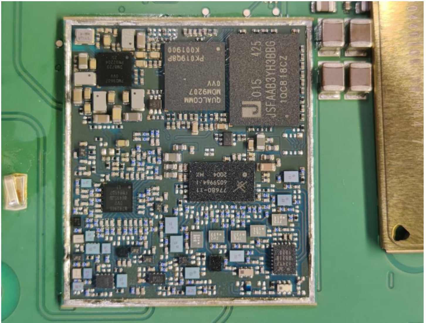
Cell Module PCB Close Up – Shield Removed
