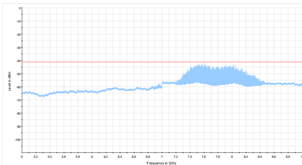
Radiates Emission from 5GHz to 9GHz
