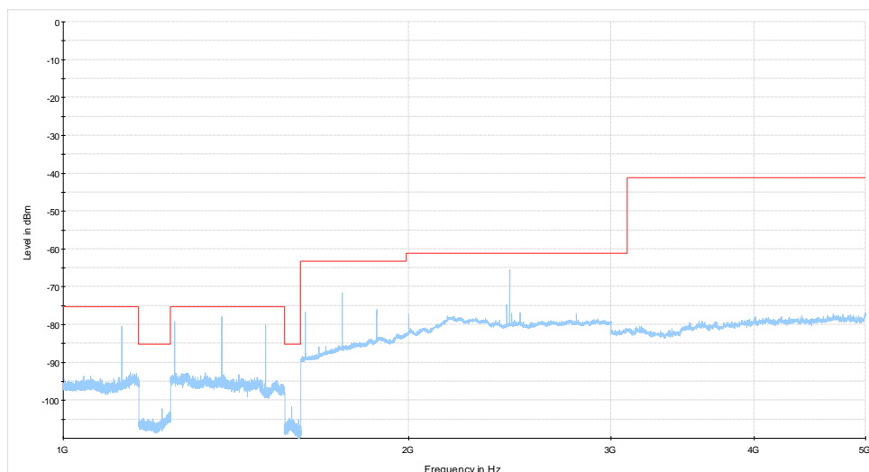
Radiates Emission from 1GHz to 5GHz
