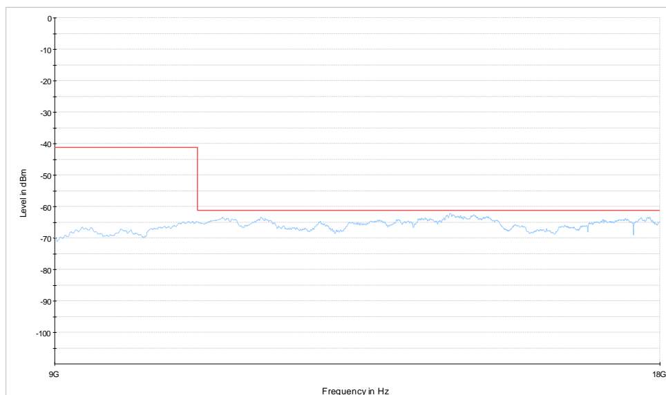
Radiates Emission from 9GHz to 18GHz
