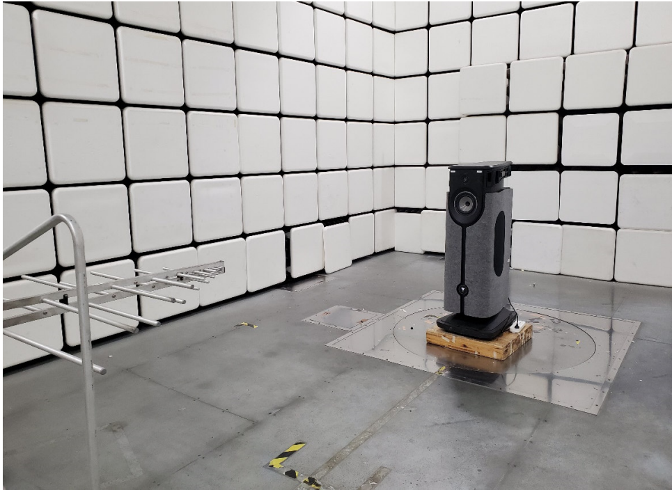
30MHz-1GHz
