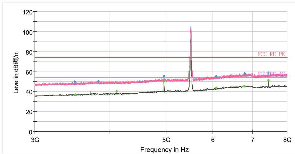
Radiates Emission from 3GHz to 8GHz
