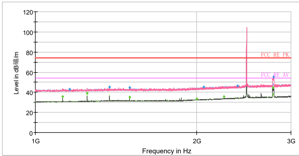
Radiates Emission from 1GHz to 3GHz
