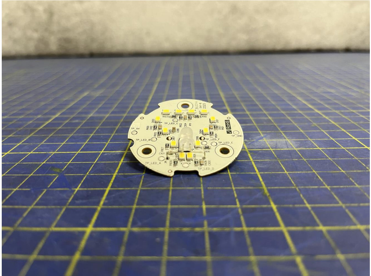
Logo PCB (Top)
