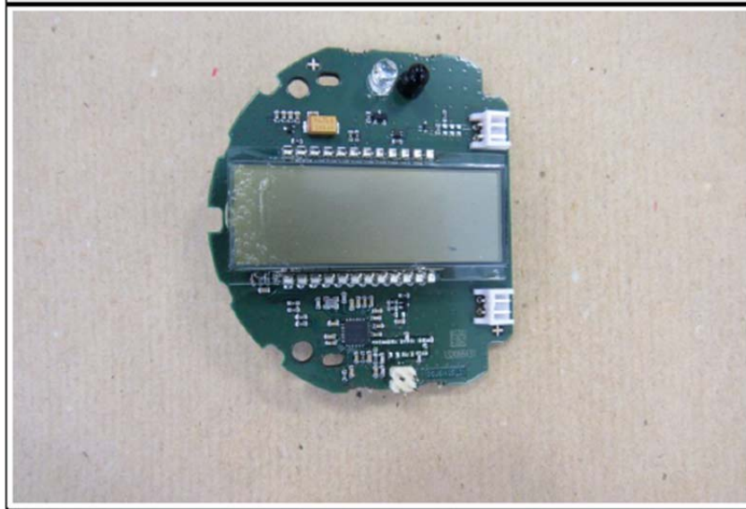
EUT PCB II front
