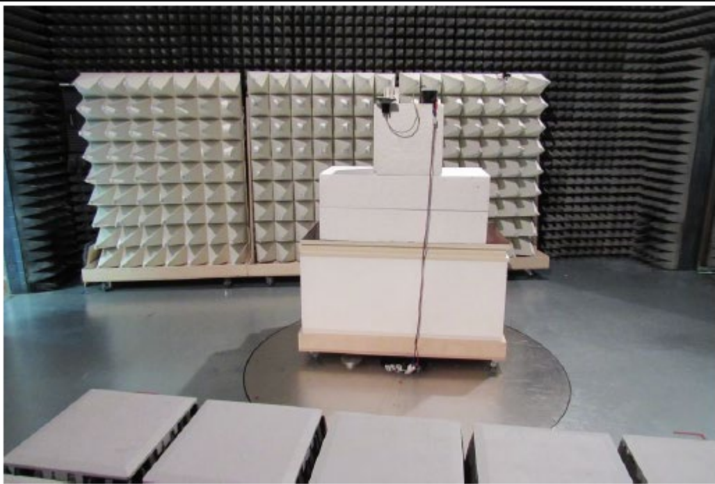
PIT ANTENNA 6697916
