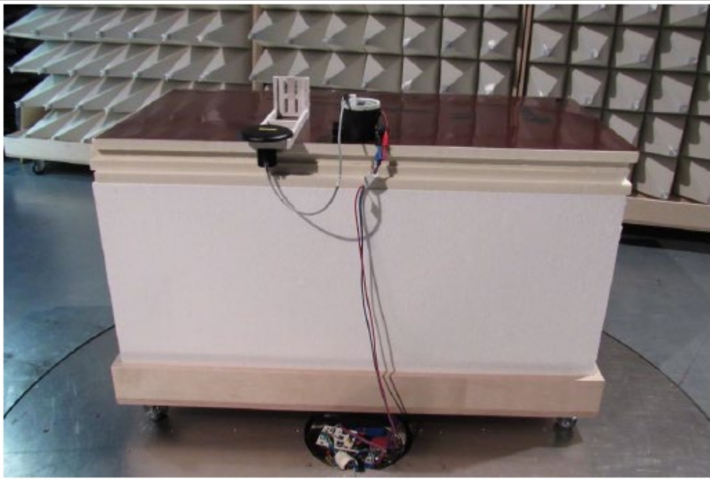
PIT ANTENNA 6697916
