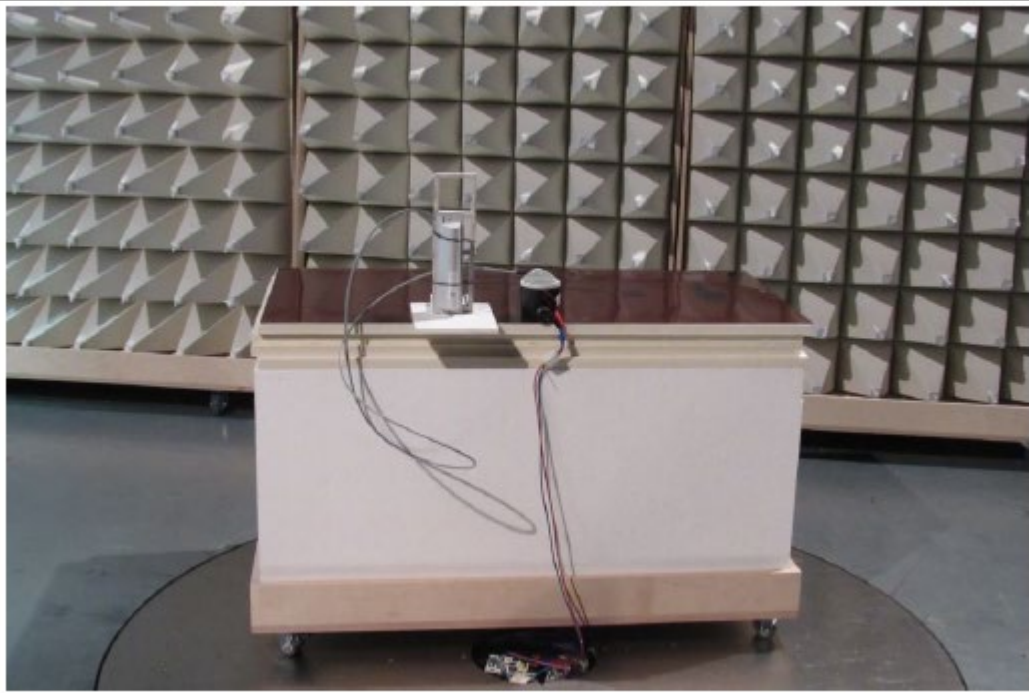
WALL ANTENNA
