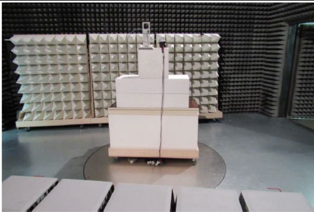
WALL ANTENNA
