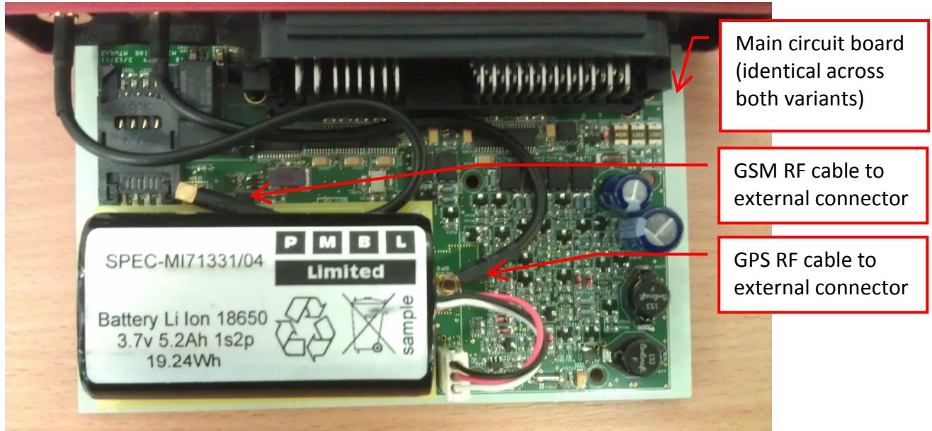
Fig 2. MTU4-B internal view
