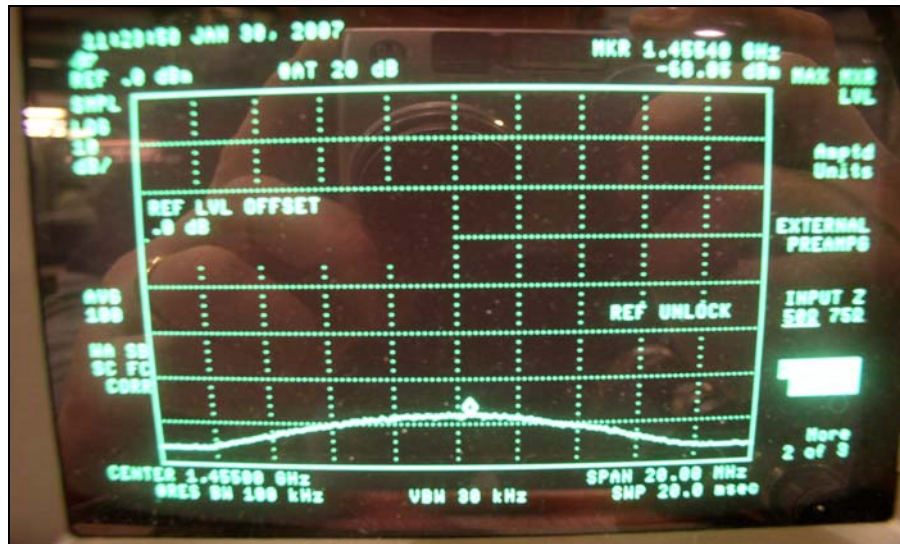
Figure 4-8C. Third Harmonic (1455 MHz) = -68.95 dBm (Pre-Filter)
