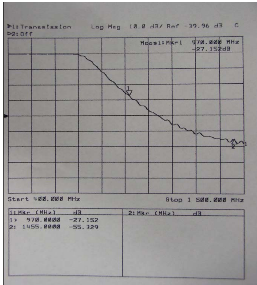
Figure 4-8D. Harmonic Filter Sweep
