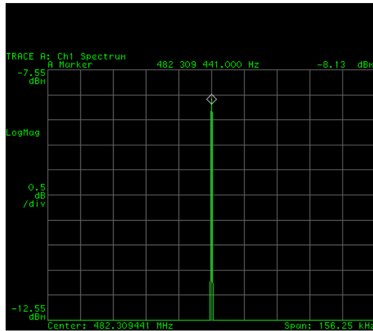
Figure 4-12. Pilot Frequency Plot
