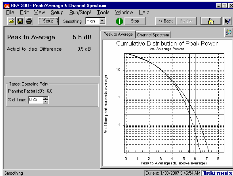
Figure 4-5. Peak to Average Plot
