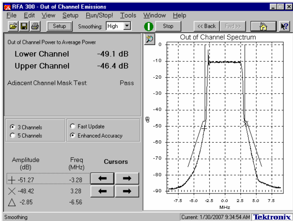
Figure 4-8E. Out of Band Emissions Plot (Post-Filter)
