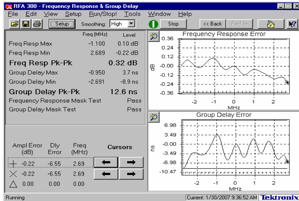
Figure 4-4. Frequency Response and Group Delay Plots
