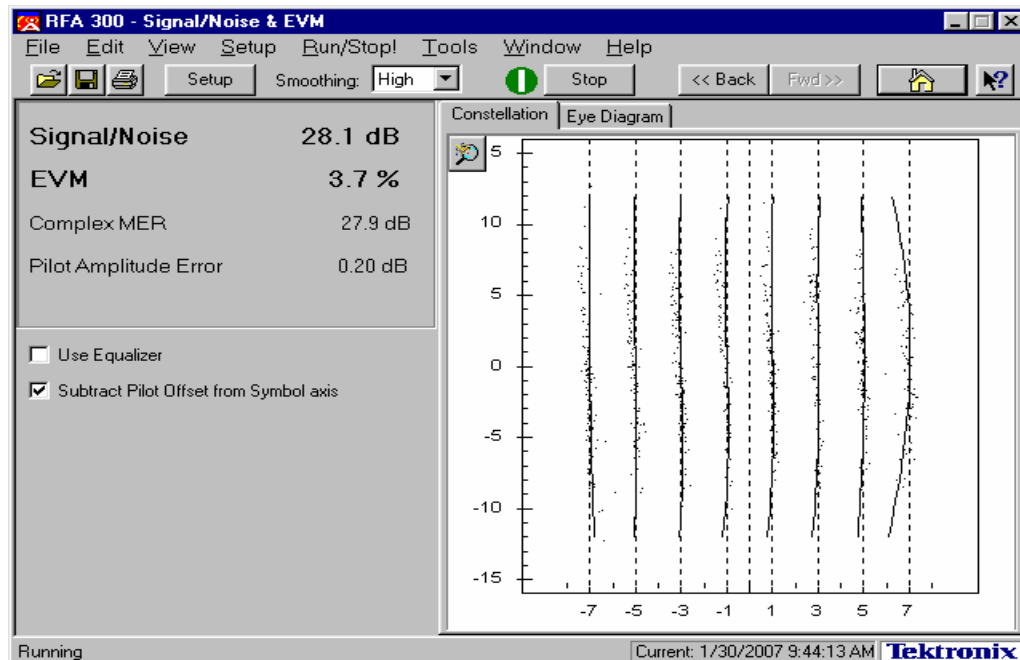
Figure 4-3B. Constellation Diagram
