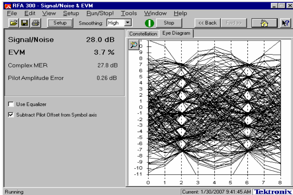
Figure 4-3A. Eye Diagram
