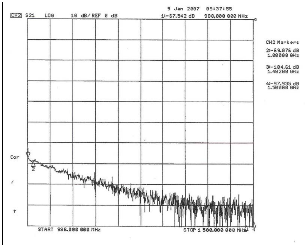
Figure 4B-8D. Harmonics
