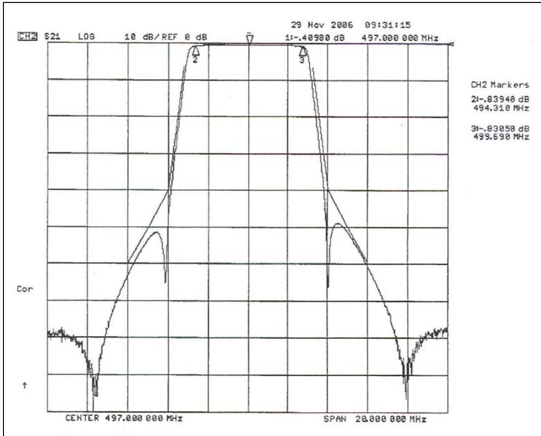
Figure 4B-8E. Bandpass Filter Response
