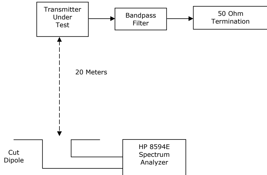
Figure 4B-9. Test Setup for Measuring Radiated Emissions
