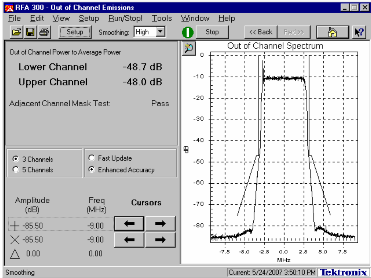
Figure 4B-8F. Out of Band Emissions Plot (Post-Filter)
