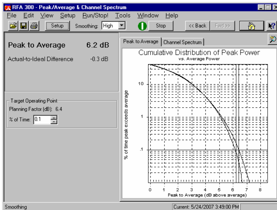
Figure 4B-5. Peak to Average Plot
