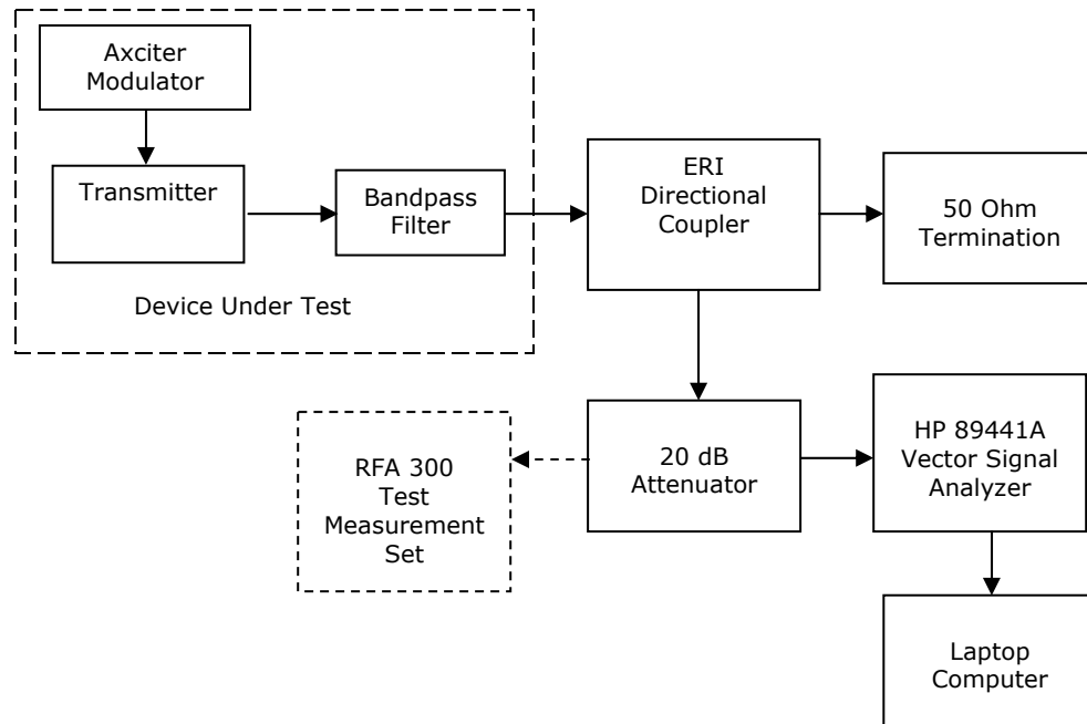
Figure 4B-2. Typical Demodulation Test Setup
