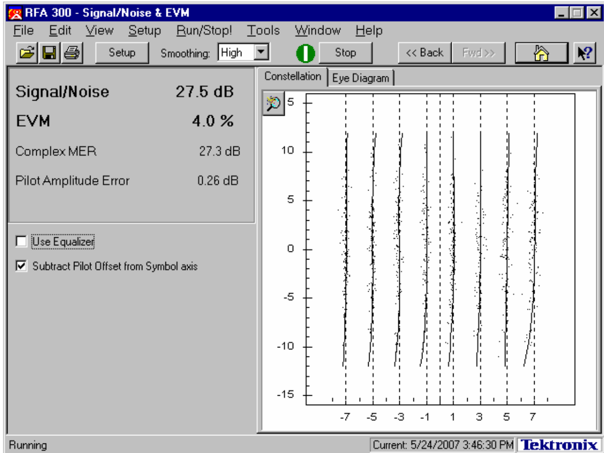
Figure 4B-3. EVM and SNR Measurement
