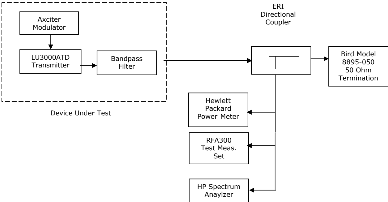
Figure 4B-1. Test Equipment Setup for RF Power Measurements
