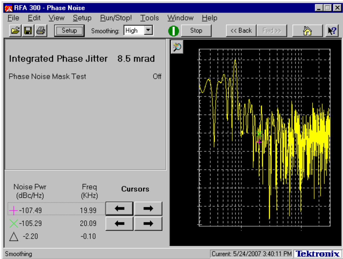
Figure 4B-6. Phase Noise Plot
