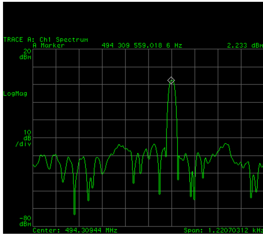
Figure 4B-12. Pilot Frequency Plot
