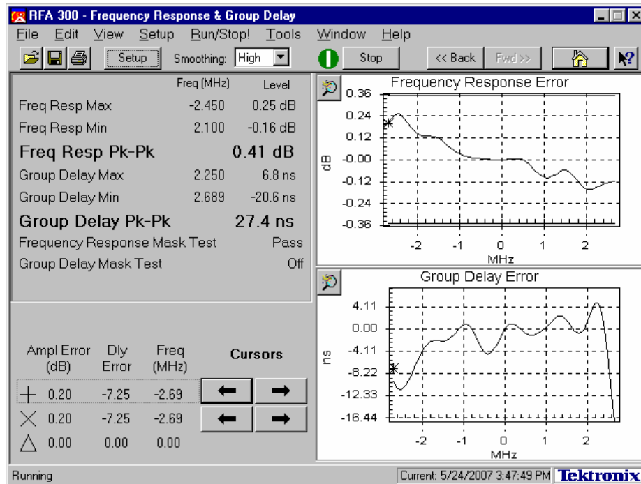
Figure 4B-4. Frequency Response and Group Delay Plots
