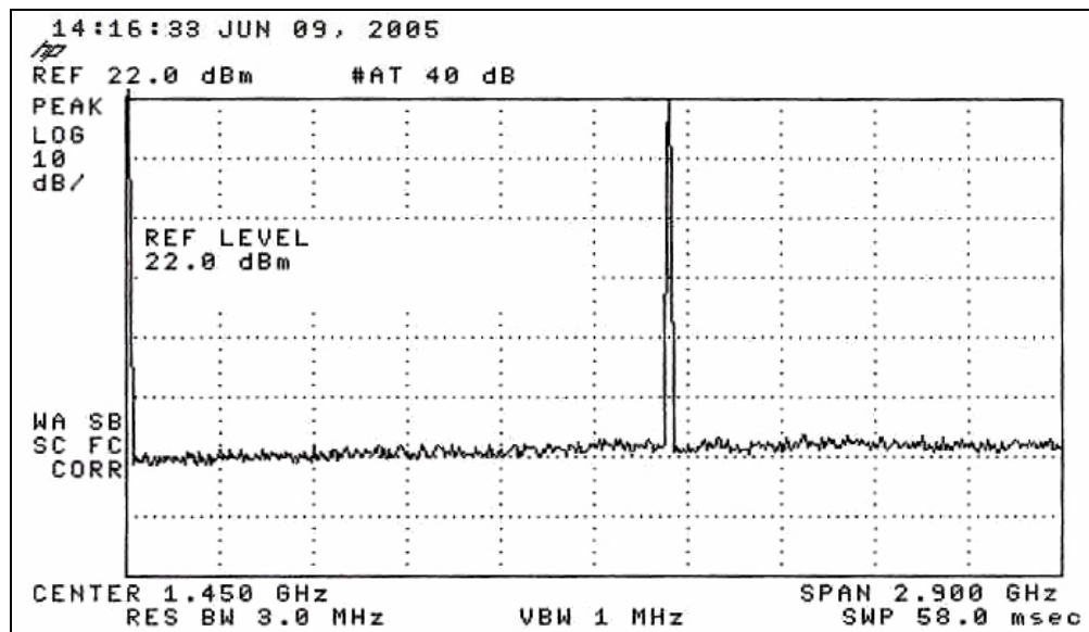
Figure 4-7. Products Above the -57 dB Noise Floor of the Spectrum Analyzer (2.900 GHz Span)
