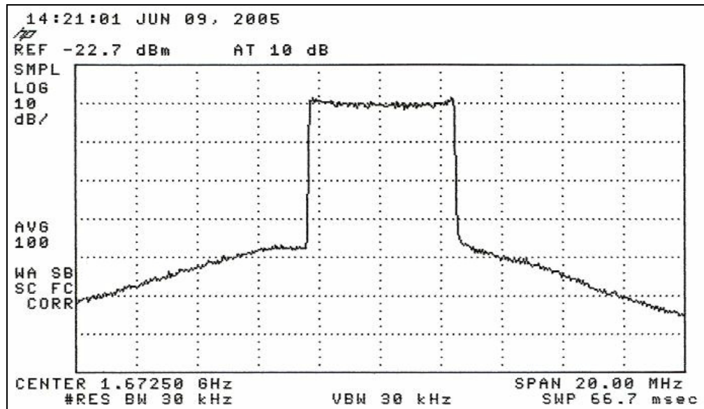
Figure 4-8. Conducted Spurious Emissions (before channel filter)
